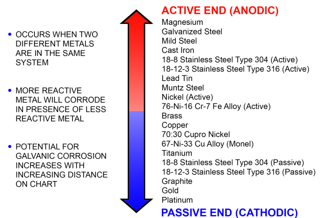
Fig. 2 Galvanic Corrosion
