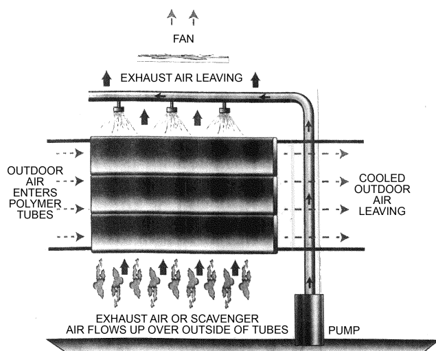
Fig. 3 Cross-Flow Plate Air-to-Air Indirect Evaporative Cooling Heat Exchanger (Munters)
