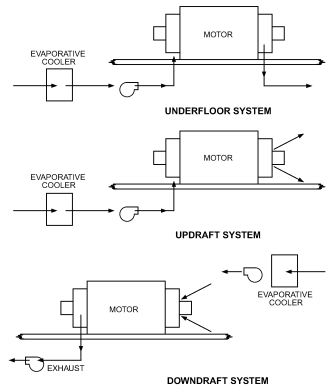
Fig. 17 Arrangements for Cooling Large Motors
