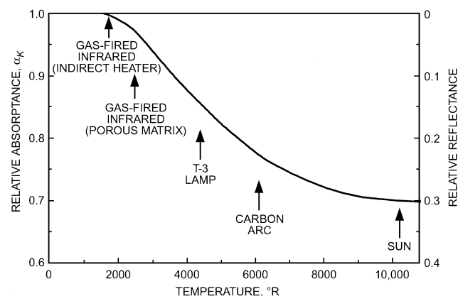
Fig. 1 Relative Absorbance and Reflectance of Skin and Typical Clothing Surfaces at Various Color Temperatures
