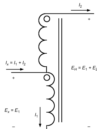
Fig. 7 Typical Autotransformer
