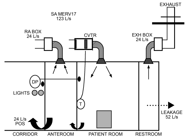
Fig. 3 Protective Environment Room Arrangement
