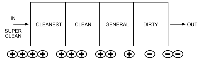
Fig. 1 Controlling Air Movement through Pressurization
