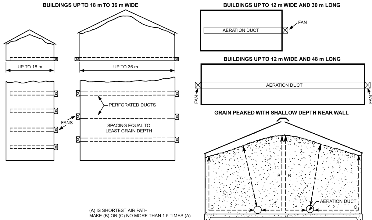
Fig. 13 Duct Arrangements for Large Flat Storages
