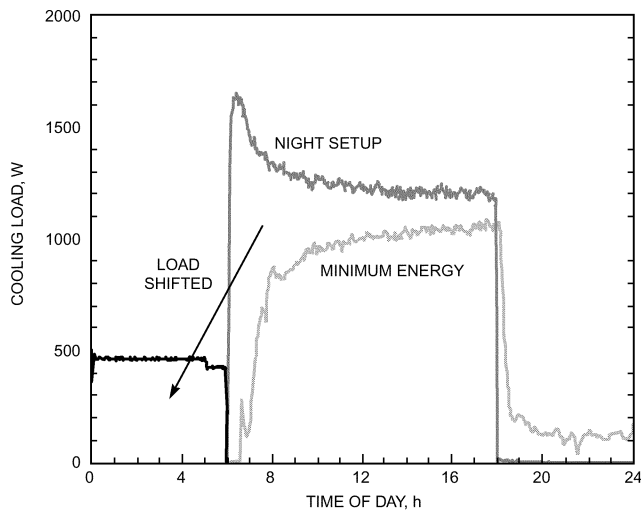
Fig. 30 Comparison of Cooling Requirements for Minimum Energy and Night Setup Control (Morris et al. 1994)
