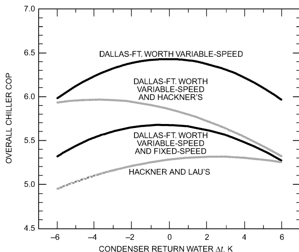
Fig. 13 Effect of Condenser Water Flow Distribution for Two Chillers In Parallel
