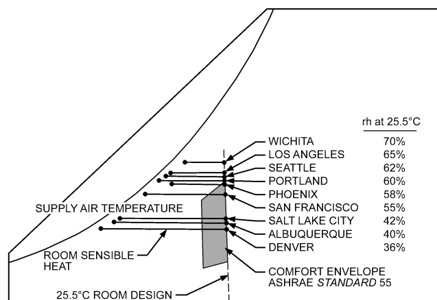
Fig. 20 Final Room Design Conditions After Two-Stage Evaporative Cooling
