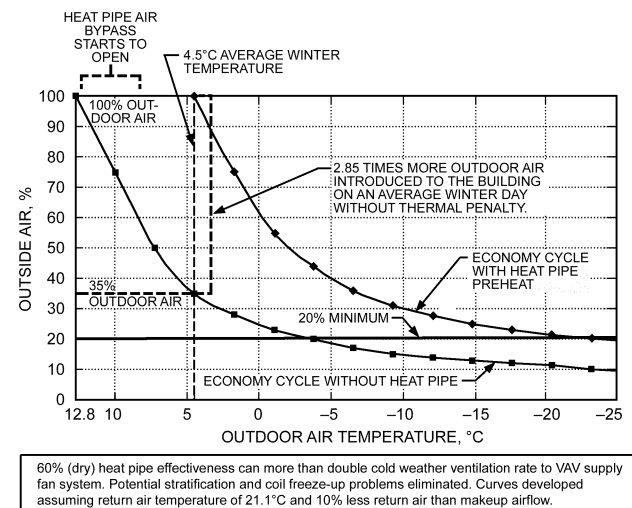
Fig. 7 Increased Winter Ventilation
