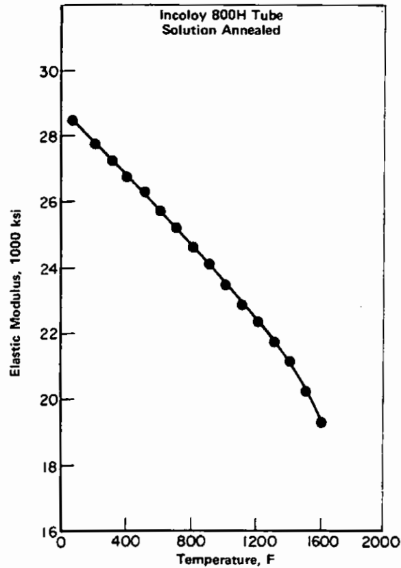
FIGURE 3.061. ELASTIC MODULUS (11, p 379)
