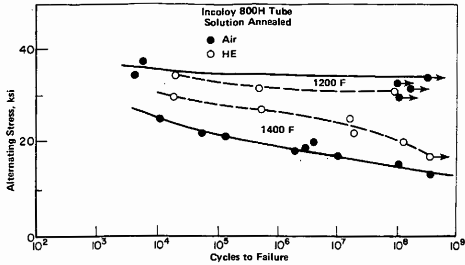
FIGURE 3.0551. HIGH-CYCLE FATIGUE AT 1200 F AND 1400 F IN AIR AND HELIUM (16, p K 23)
