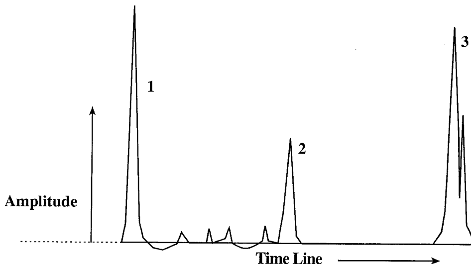
Figure 1.3: A Scan display – (1) front surface pulse signal, (2) discontinuity signal, and (3) back reflection signal
