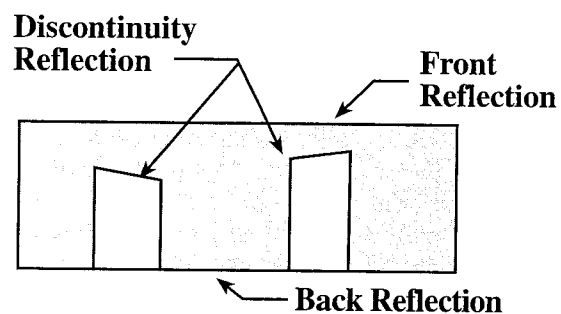
Figure 1.4: B Scan display
