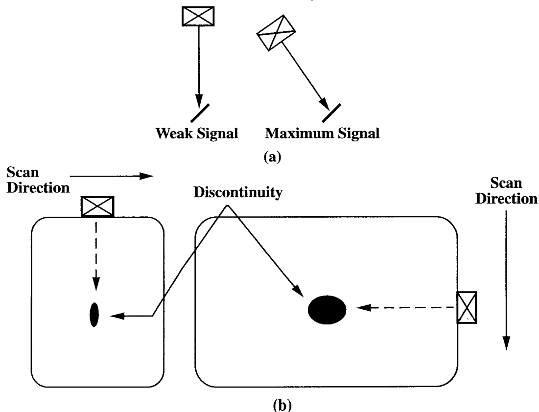
Figure 1.19: (a) angulation of search unit for maximum response, (b) testing from two surfaces to obtain maximum response
