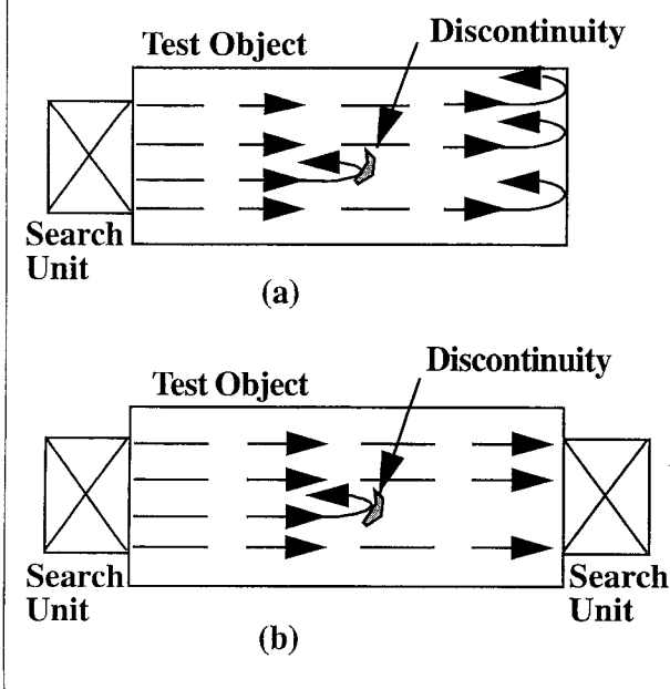
Figure 1.7: Ultrasonic test techniques — (a) pulse echo technique, (b) through transmission technique
