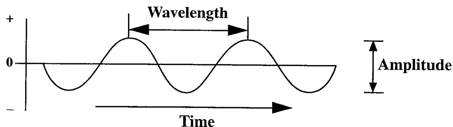
Figure 1.1: Sound wave
