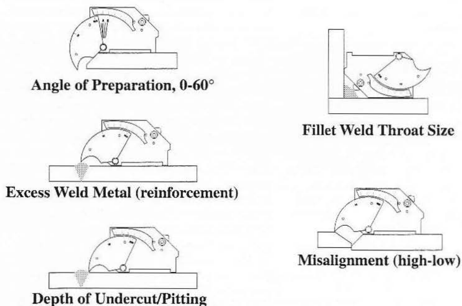
Figure 1.14: Cambridge gage
