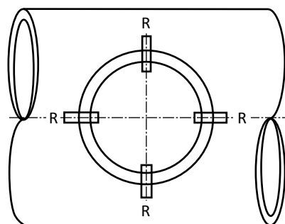
Branch weld
