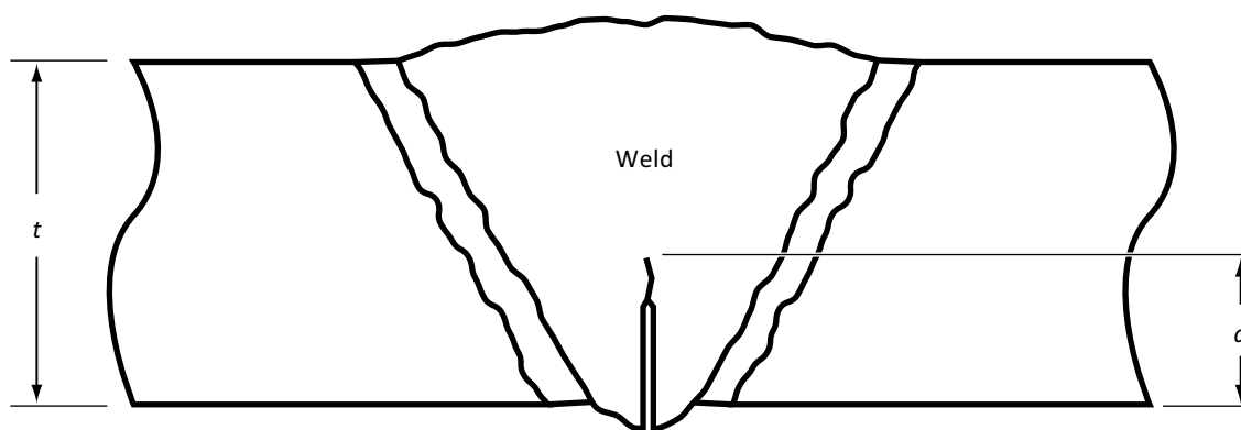
Figure K.2 Notch position for subsidiary geometry specimens (Group 3) (See Table K.2.)
