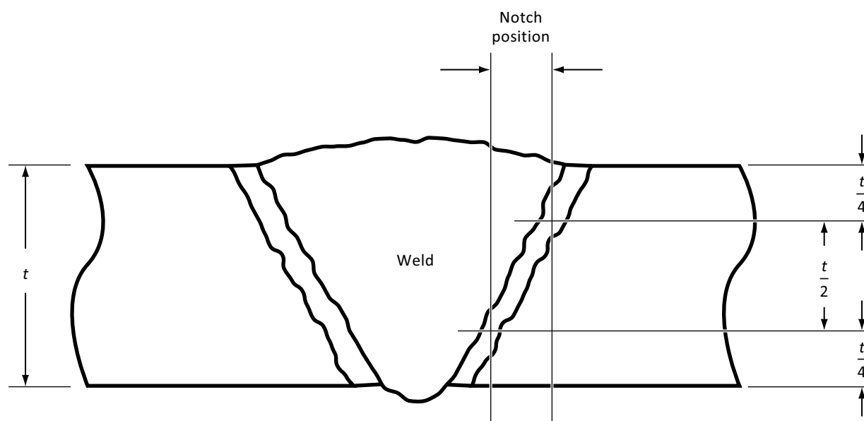
Figure K.1 Range of positions for the notch in Group 2 specimens (See Table K.2.)
