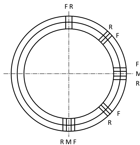
Sleeve weld (end view)
