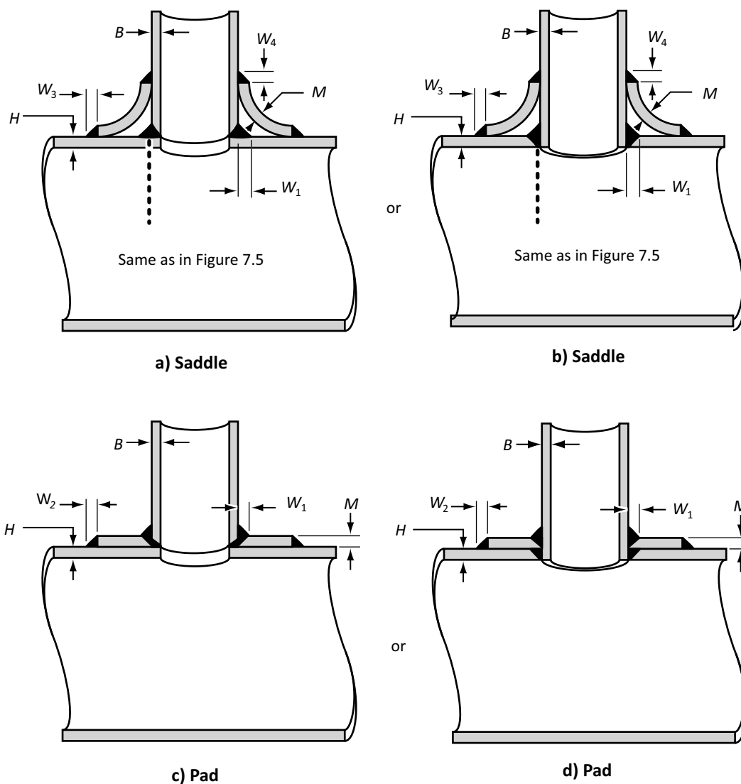
Figure 7.4 Welding details of opening with localized type of reinforcement (See Clauses 4.3.18, 4.3.19, and 7.3.2.)
