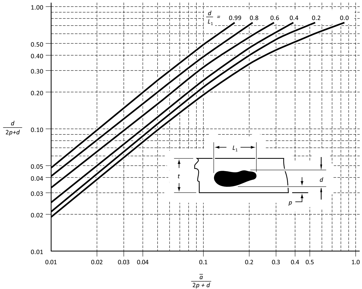
Figure K.5 Relationship between actual dimensions and \left(\frac{\bar{a}}{2p+d}\right) for embedded imperfections (See Clauses K.5.3.1.2, K.5.3.3.3, and K.5.3.4.2.)
