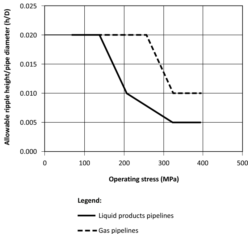
Figure 10.6 Recommended maximum allowable ripples, wrinkles and buckles for steel pipe (See Clause 10.10.8.3.)
