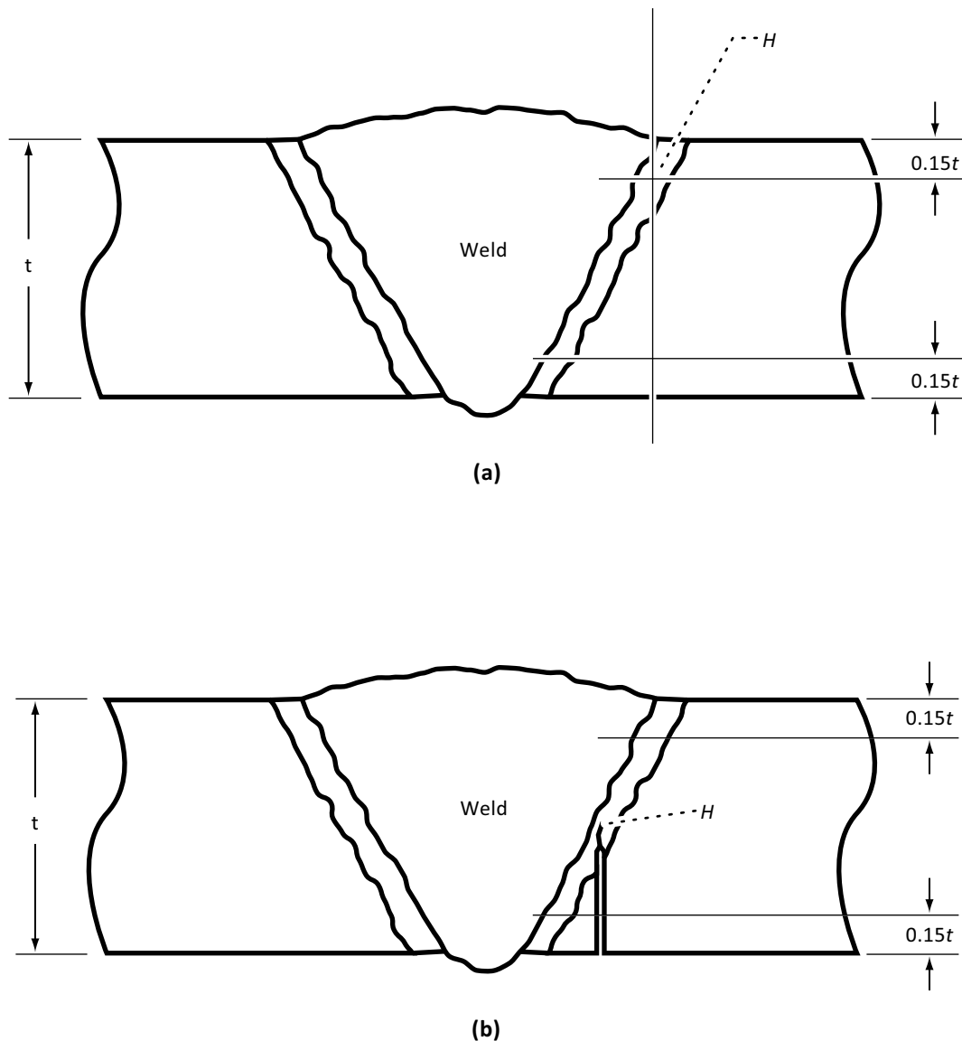
Figure K.3 Specimen notch positions for Group 4 tests (See Table K.2.)
