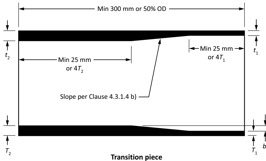
Figure 4.1 Example of transition piece dimensions (See Clause 4.3.1.4.)
