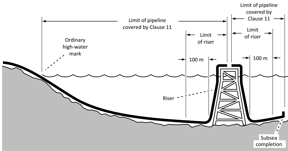
Figure 11.2 Subsea completion to platform and platform to shore (typical arrangement) (See Clause 11.1.1 and Figure 11.1.)
