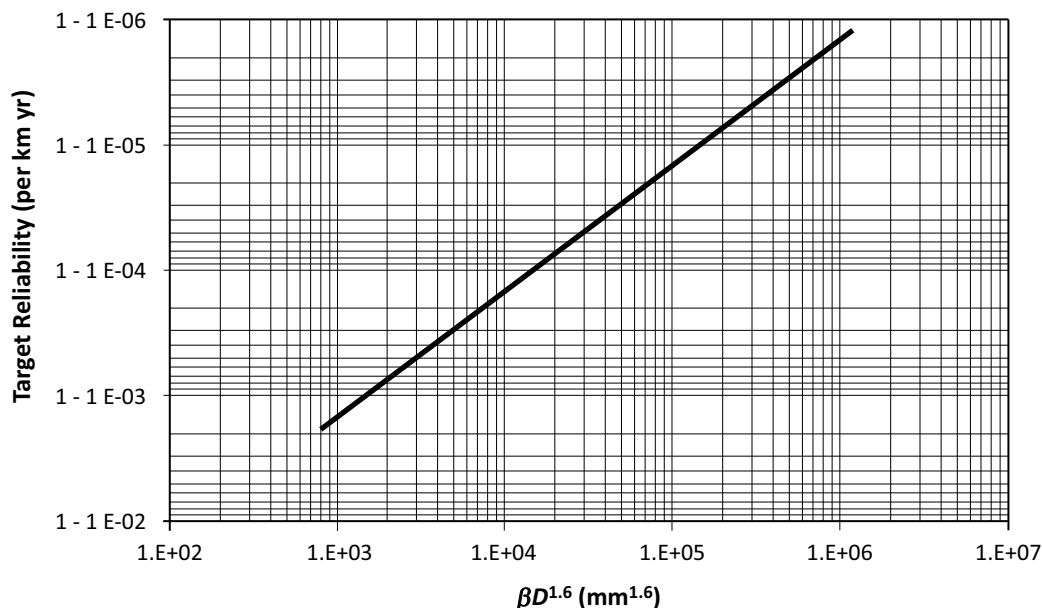
Figure O.4 LVP liquid hydrocarbon pipeline target reliability for ultimate limit states (See Clause O.1.5.2.3.1.)
