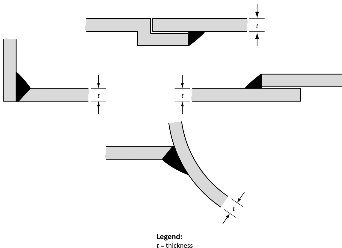
Figure 7.14 Root-break or macrosection test specimens (See Clauses 7.7.7.1 and 7.7.8.2.)
