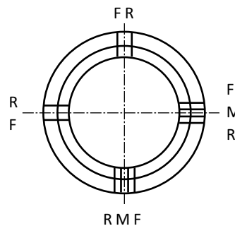
Sleeve weld (end view)
