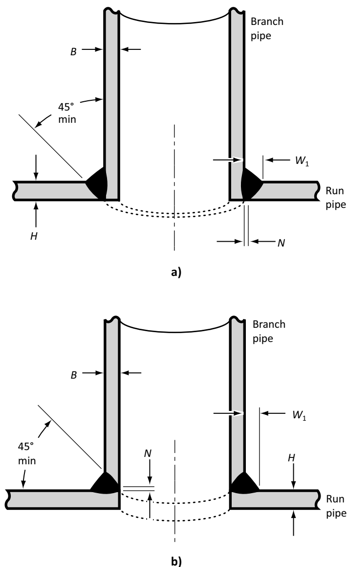
Figure 7.5 Welding details for branch-to-run pipe connection (See Clauses 4.3.19, 7.3.2, 12.7.3.3 and Figures 4.3 and 7.4)
