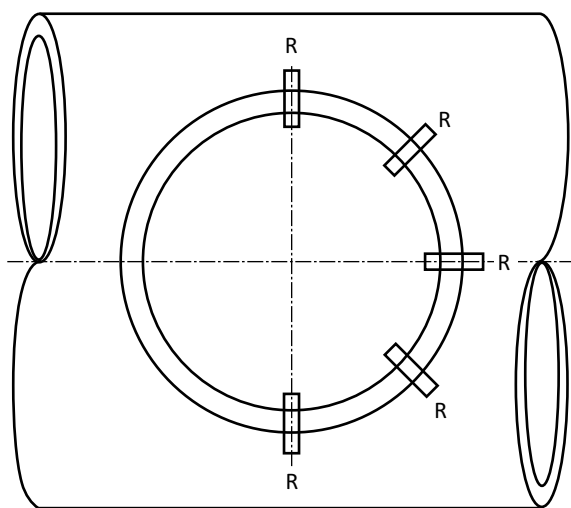
Branch weld
