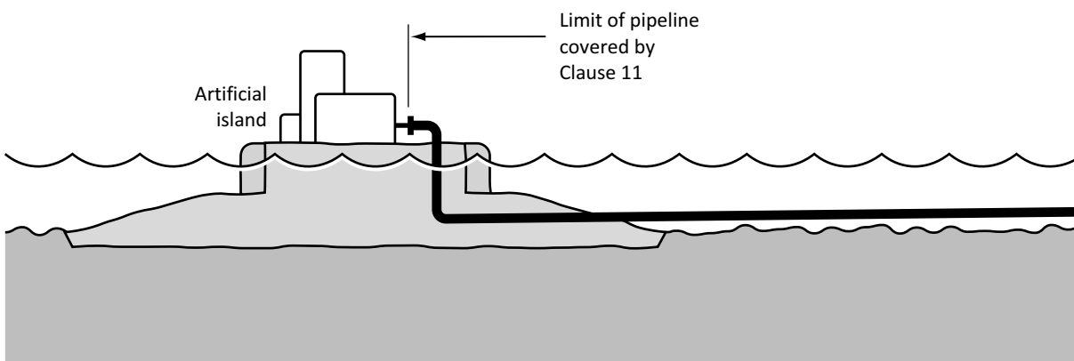
Figure 11.4 Artificial island (typical arrangement) (See Clause 11.1.1 and Figure 11.1.)
