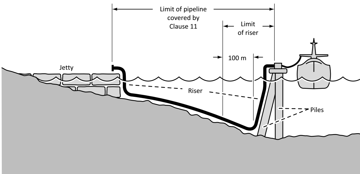
Figure 11.3 Landward jetty system and offshore loading/unloading system (typical arrangement) (See Clause 11.1.1 and Figure 11.1.)
