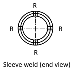
Sleeve weld (end view)
