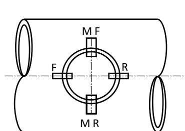
Branch weld
