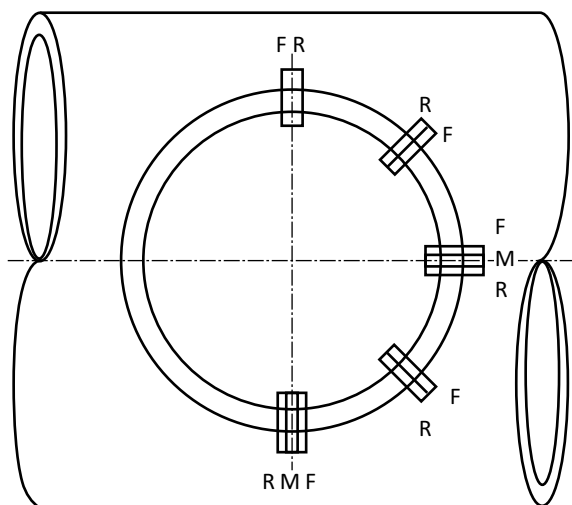
Branch weld
