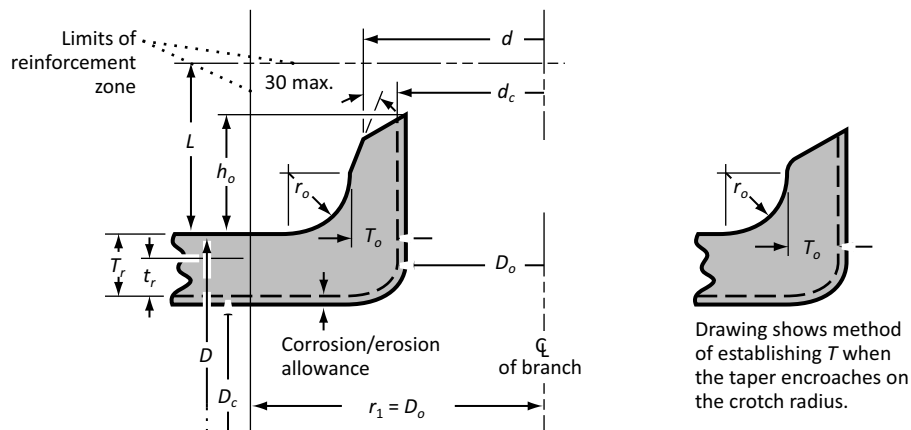
Figure 4.3 Integrally reinforced extruded outlet headers (See Clause 4.3.17.)
