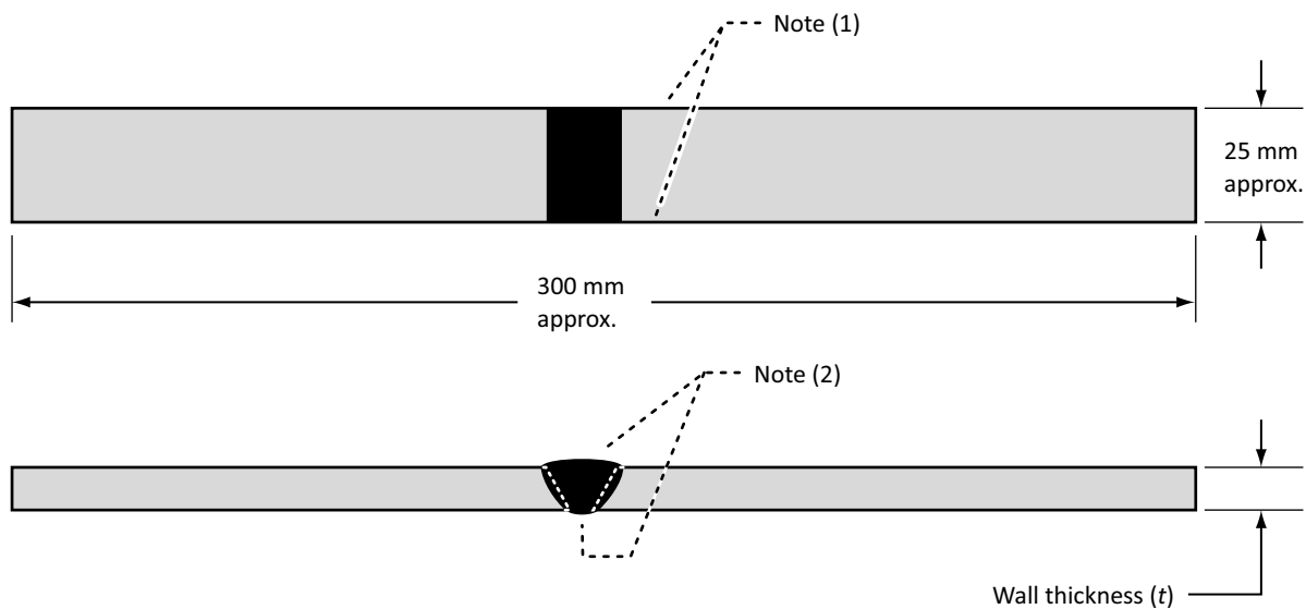
Figure 7.7 Tension test specimen (See Clauses 7.7.2.1 and 7.7.3.1.)
