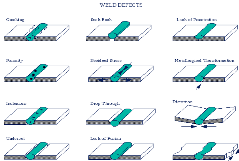
Figure 9.3 Various Types of Weld Defects
