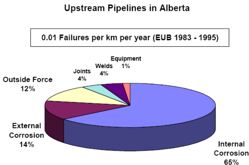
Figure 6.2 History of Upstream Pipeline Failures and Failure Causes in Alberta, Canada
