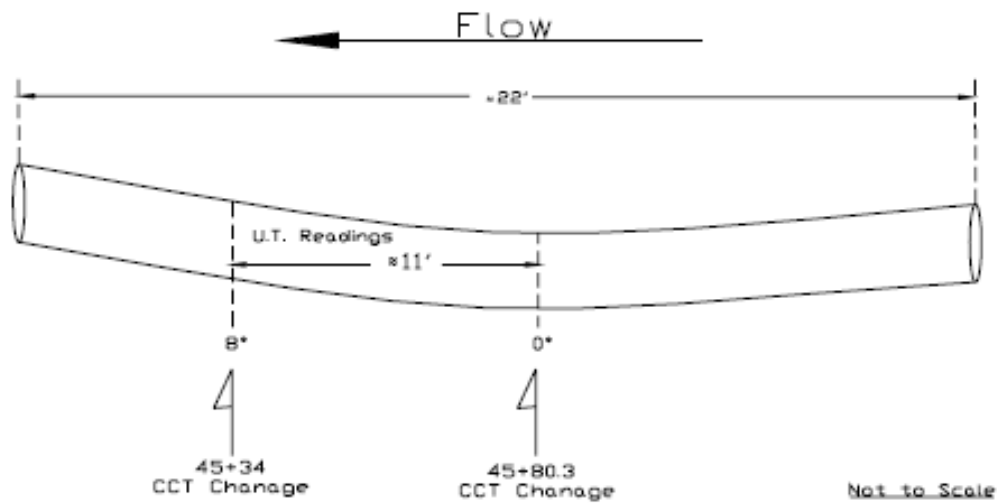
Figure 13.9 Schematic of Pipe Elevation at DG-ICDA Site 5
