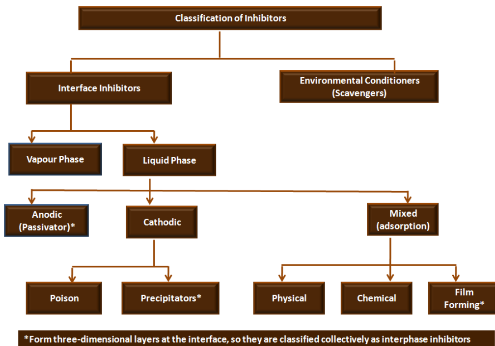
Figure 2.30 Classification of Inhibitors
