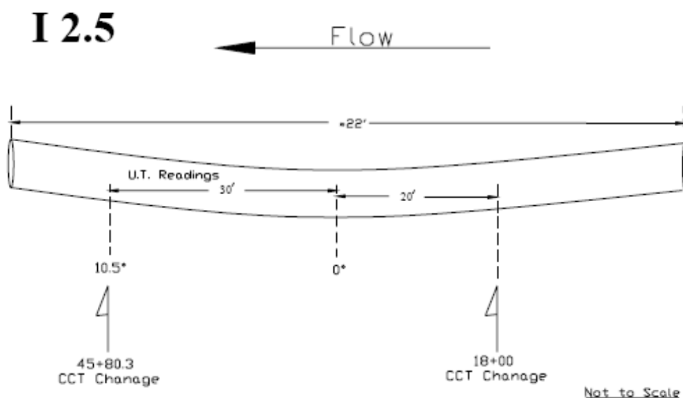
Figure 13.5 Schematic of Pipe Elevation at DG-ICDA Site 3
