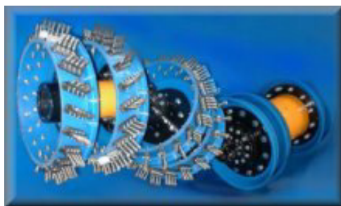
Figure 7.2 Utility Pigs: Cleaning and Sealing Pig
