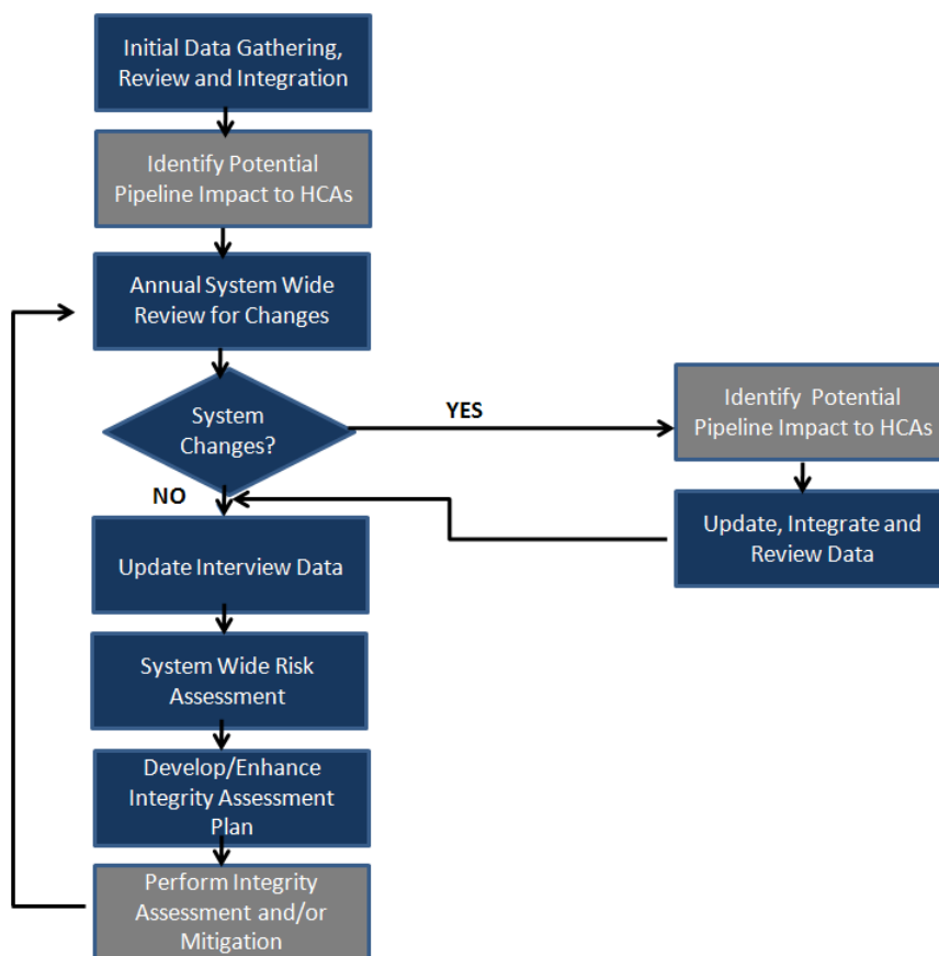
Figure 3.2 Integrity Management Process Based on API 1160 6
