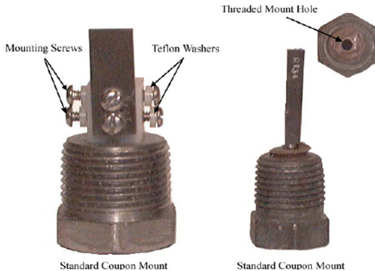
Figure 2.26 Types of Coupon Mounts
