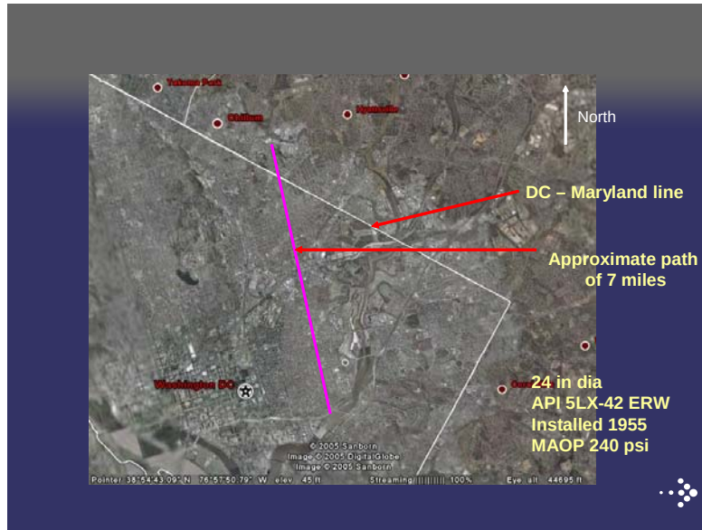
Figure 13.12 ECDA Segment
