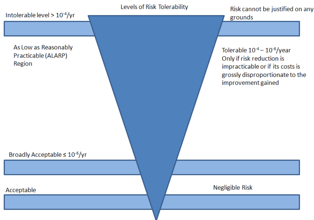
Figure 6.6 Principle of “As Low As Reasonably Practicable” (ALARP) (Source: Pigging Products and Services Association, 2004)
