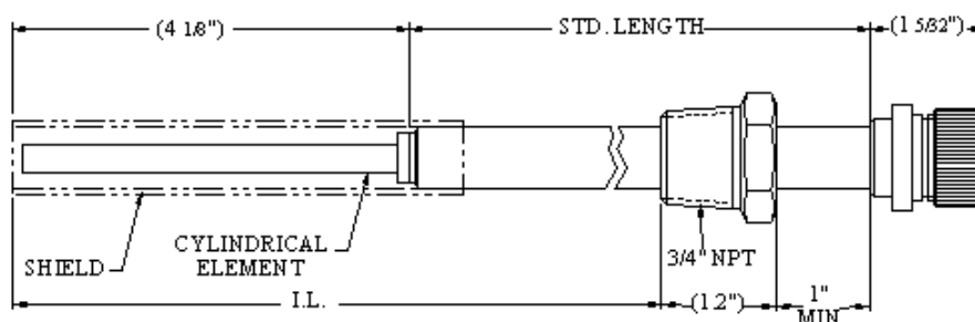
Figure 2.27 ER With Cylindrical Element, Fixed Length With \frac{3}{4} NPT Pipe Plug
