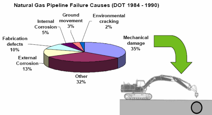
Figure 6.1 History of Natural Gas Transmission Pipeline Failures and Failure Causes in the U.S.
