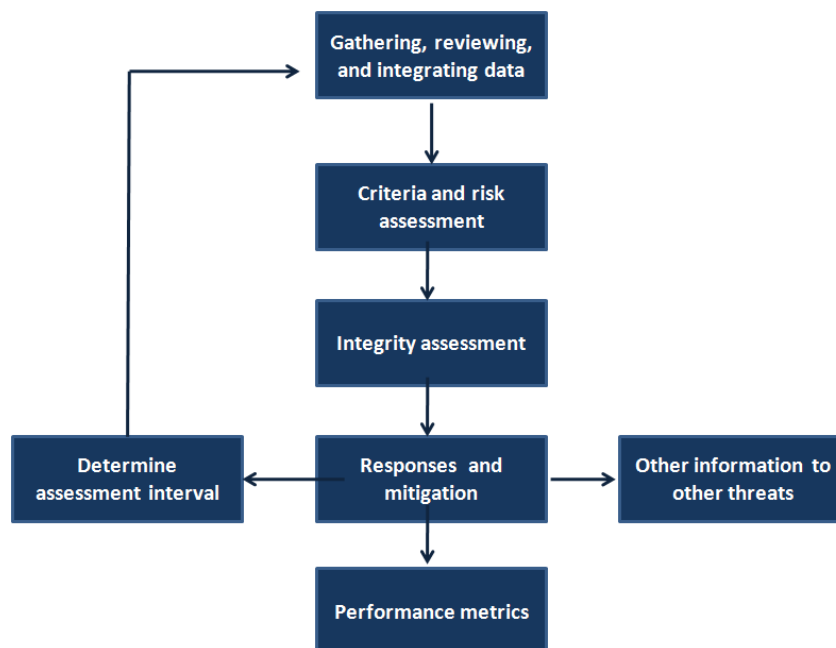
Figure 1.2 Prescriptive Integrity Management Plan, Manufacturing Threat, Construction Threat
