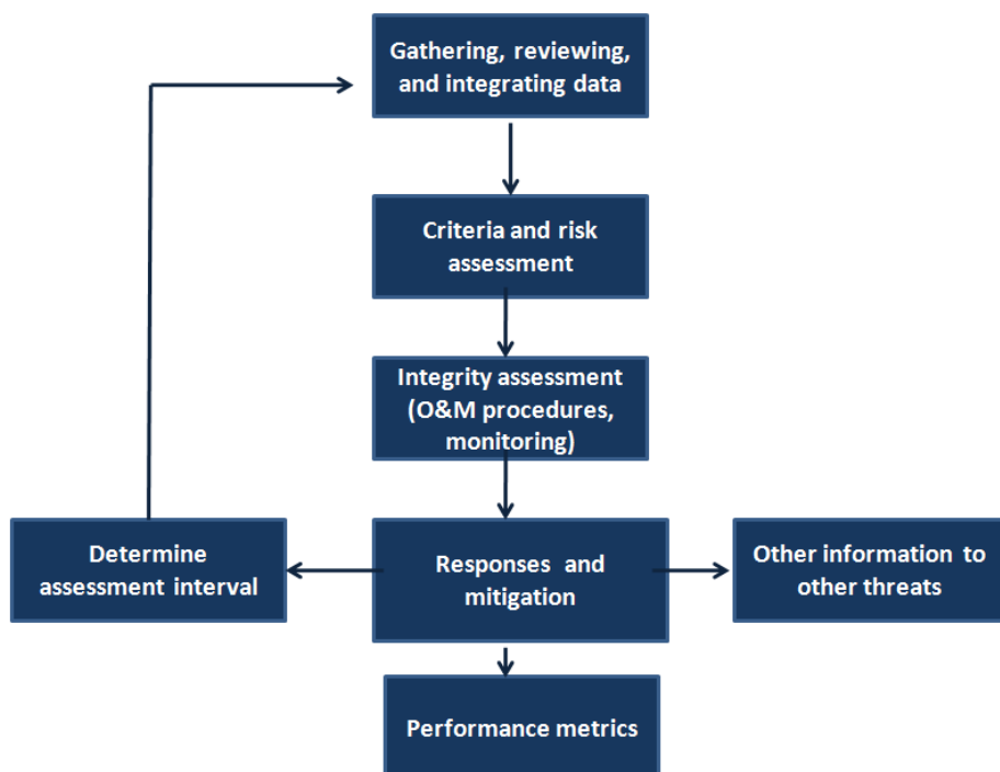
Figure 1.5 Prescriptive Integrity Management Plan, Weather-related and Outside Force Threat
