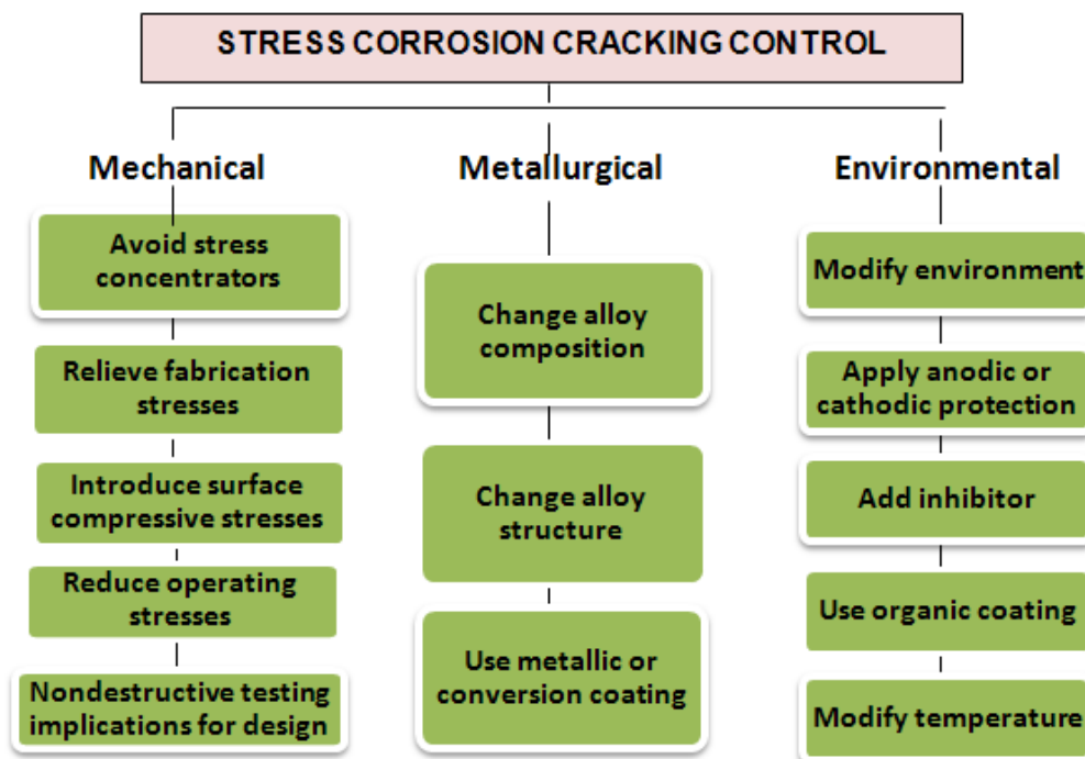
Figure 2.21 Key Stress Corrosion Cracking Control Methods
