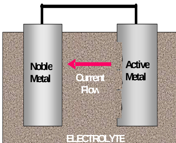
Figure 2.18 Galvanic Corrosion Cell
