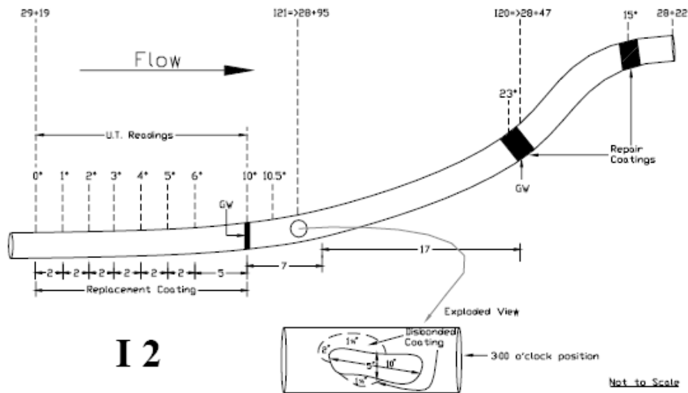
Figure 13.3 Schematic of Pipe Elevation at DG-ICDA Site 2
