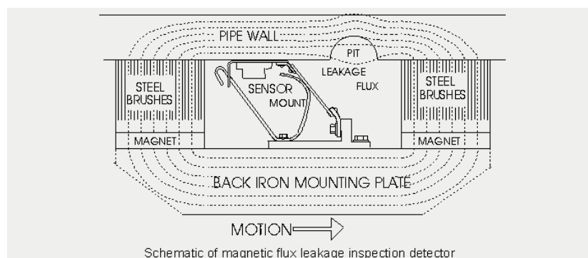
Figure 7.9 MFL Schematic Diagrams
