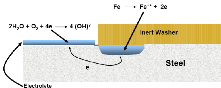
Figure 2.8 A Schematic Illustration of a Typical Crevice Corrosion Cell
