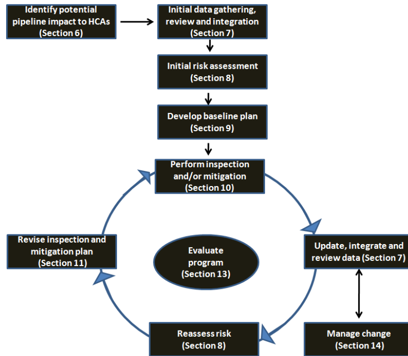
Figure 4.2 Framework for an Integrity Management Program
