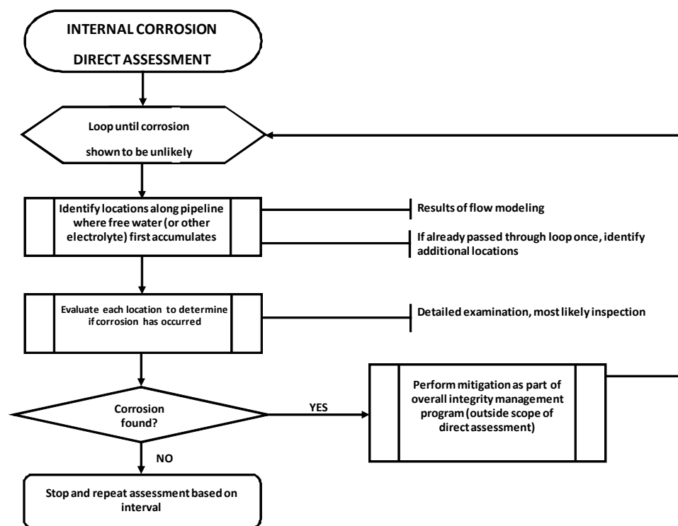
Figure 7.12 Internal Corrosion Direct Assessment
