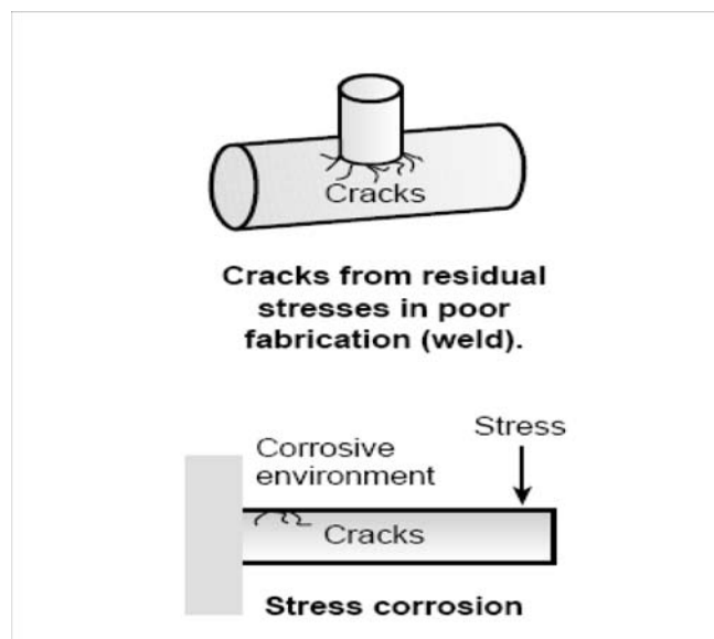
Figure 2.22 A Schematic Illustration of Stress Corrosion Cracking
