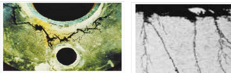
Figure 2.12 Intergranular Cracking and Transgranular Cracking (micrographs and SEM images)
