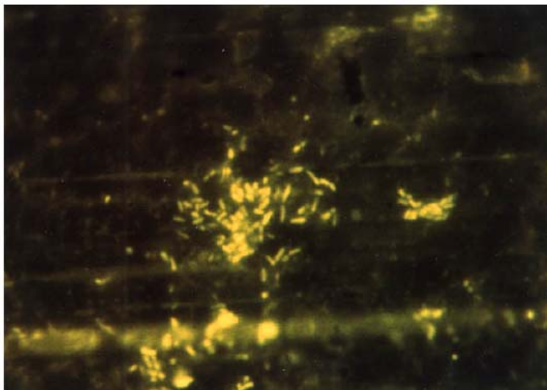
Figure 2.11 A Fluorescent Microscopic Examination of a Surface “Replica” of Bacteria Colony Associated With Corrosion Products
