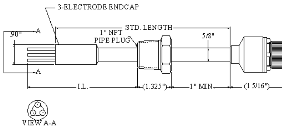
Figure 2.28 Three-Electrode LPR with Fixed length and a 1-Inch NPT Pipe Plug
