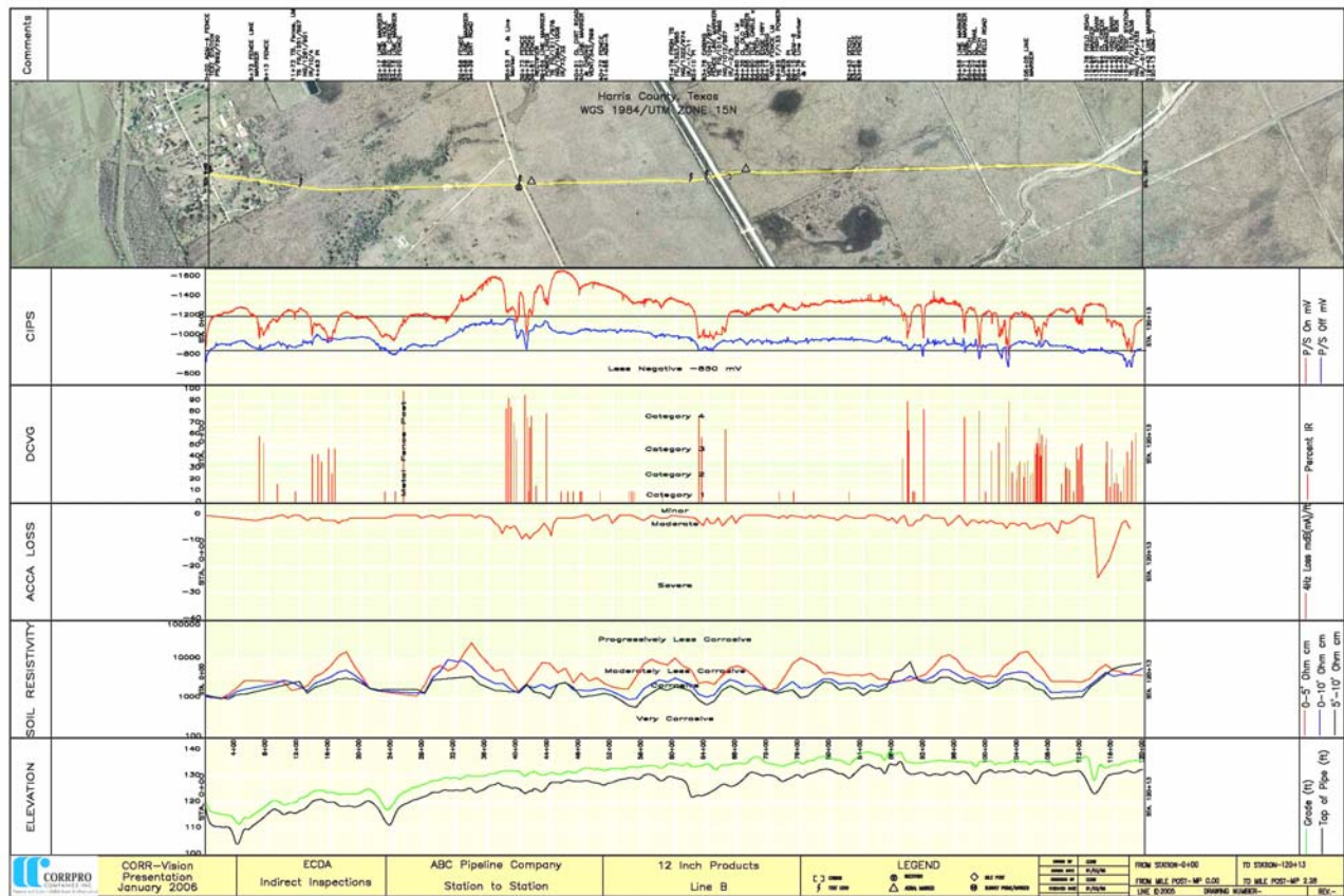
Figure 5.1 Combined Inline Inspection and External Corrosion Direct Assessment Chart
