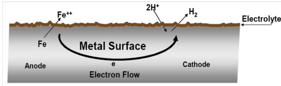
Figure 2.5 Anode-Cathode Regions on a Pipeline and the Corrosion Chemistry
