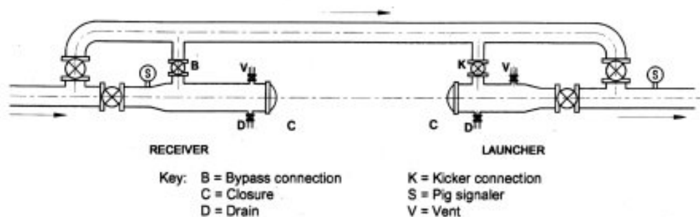
Figure 7.11 Pig Launcher and Receiver
