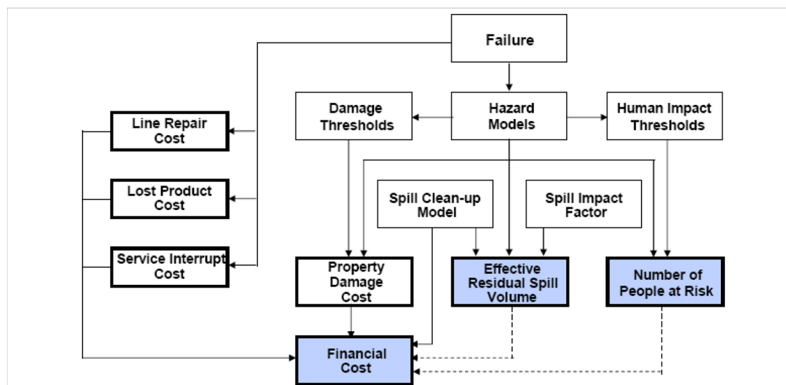
Figure 6.4 A Schematic Flow-Chart for Quantification of Consequences of Pipeline Failure
