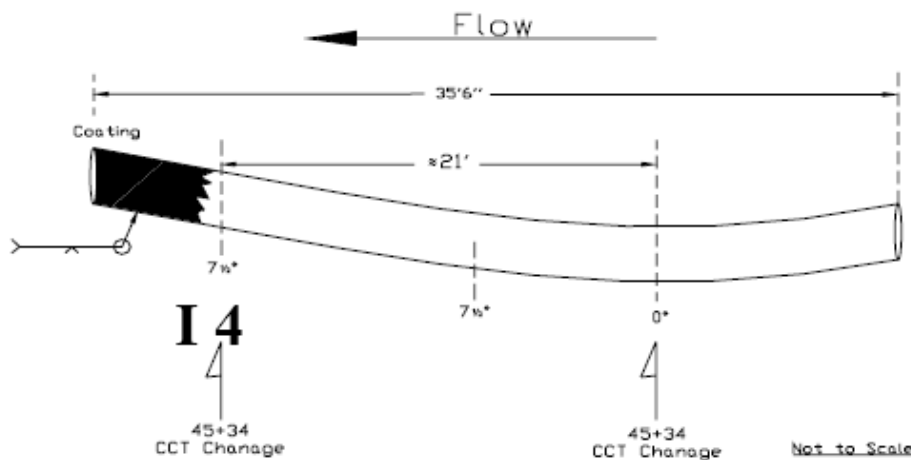
Figure 13.7 Schematic of Pipe Elevation at DG-ICDA Site 4
