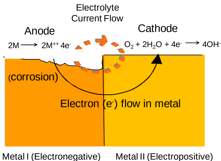
Figure 2.9 A Schematic of a Bimetallic System Illustrating Galvanic Corrosion
