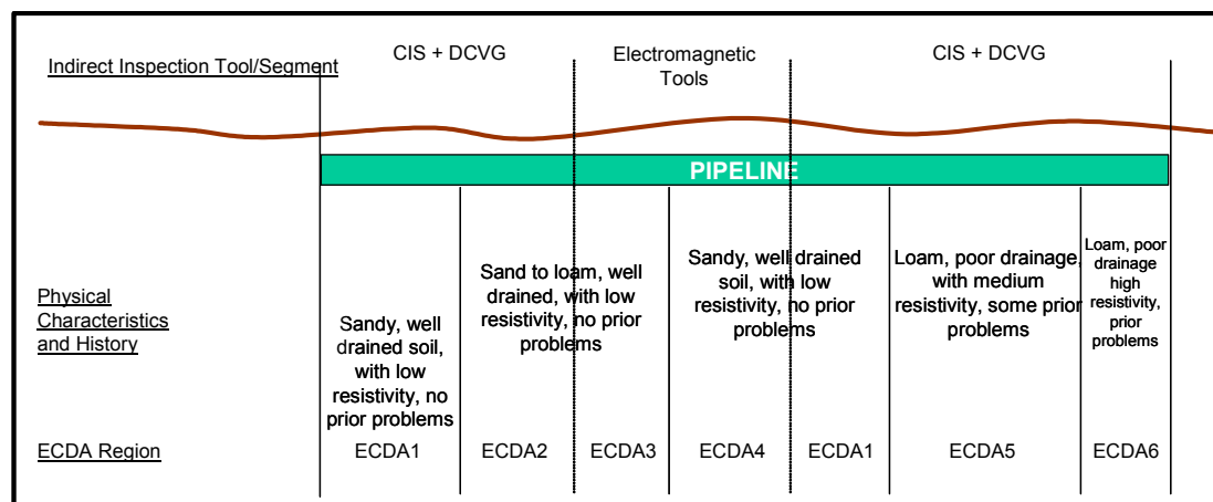
Figure 4.4 Illustration of ECDA Region Definitions
