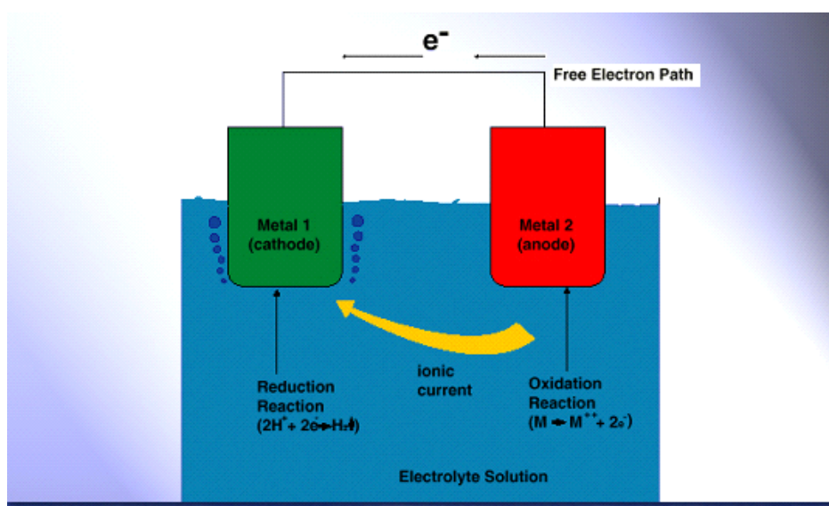
Figure 2.2 Four Conditions for Corrosion to Occur
