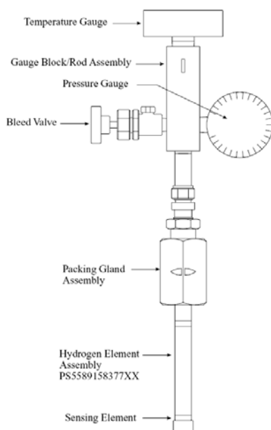
Figure 2.29 Hydrogen Probe With Retractable Packing Gland Assembly
