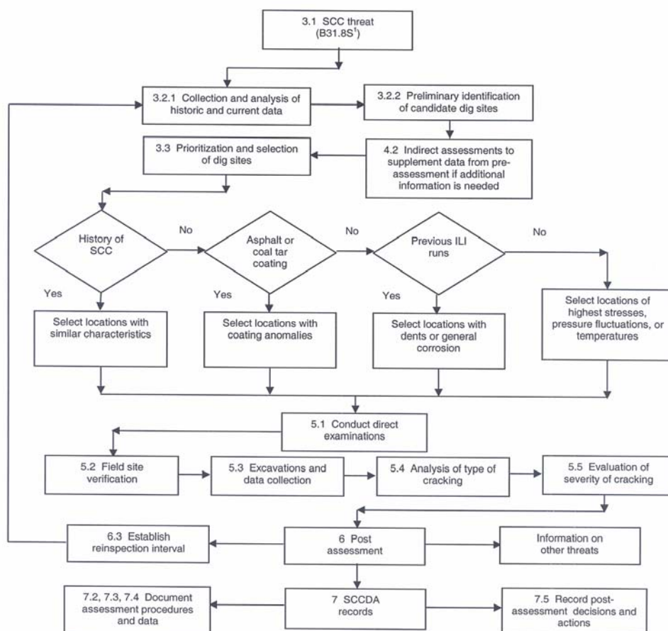
Figure 2.24 A Flow Chart for SCCDA Process (numbers refer to the paragraph numbers in NACE Standard SP0204)
