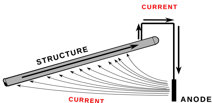
Figure 2.17 Typical Galvanic Anode Cathodic Protection
