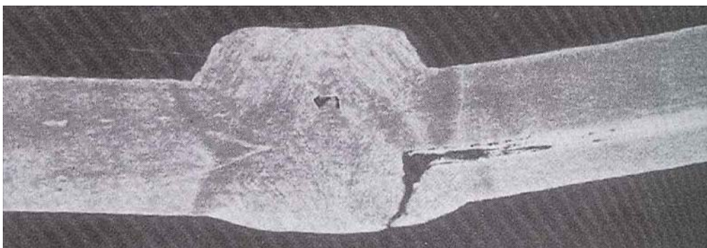
Figure 9.2 Cracking in a Weld Deposit Caused by Lamination in Steel Base Metal
