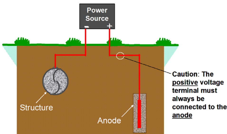
Figure 2.19 Typical Impressed Current Cathodic Protection
