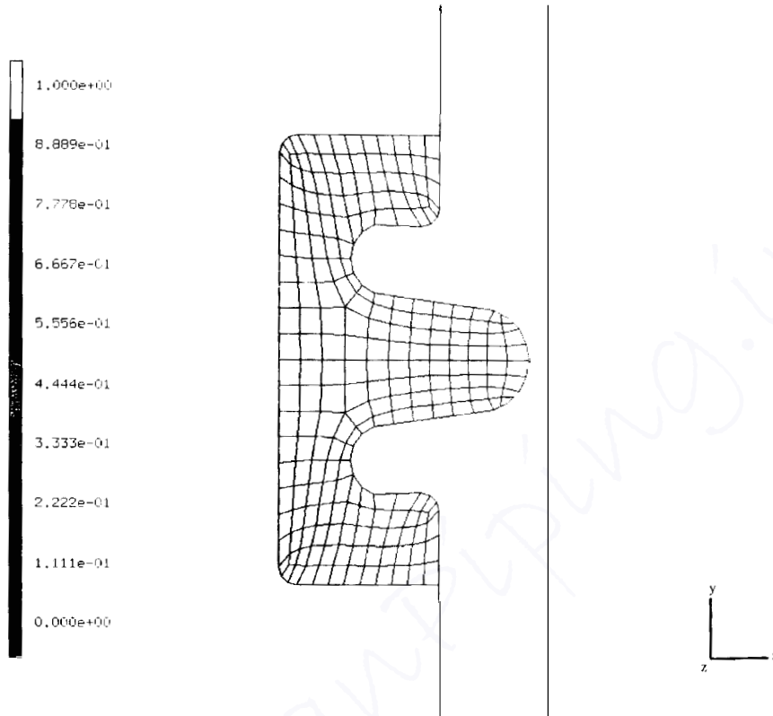
Figure 8.4 An FEA of the uncompressed molded bead
