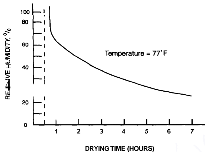
Figure 9.4 Drying time versus relative humidity for an RTV silicone.
