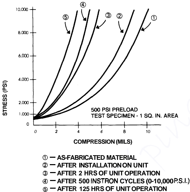
Stress versus compression: Effect of load applications
