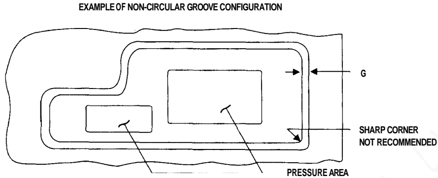
Figure 6.11 Example of a noncircular groove configuration.
