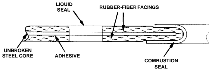
Figure 10.9 Unbroken metal core gasket.
