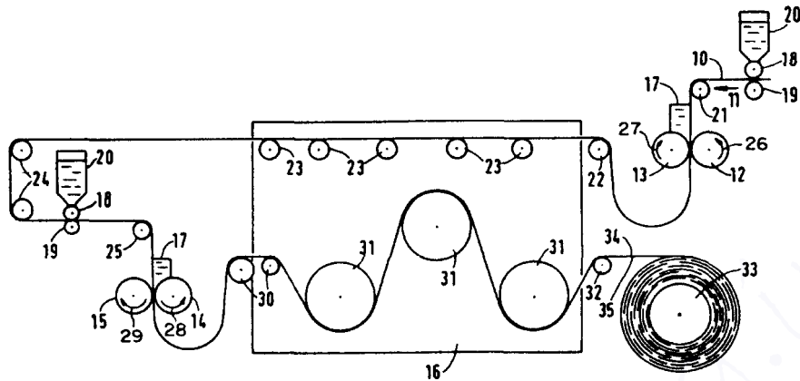
Figure 1.6 Nonstick nonasbestos perforated core process.
