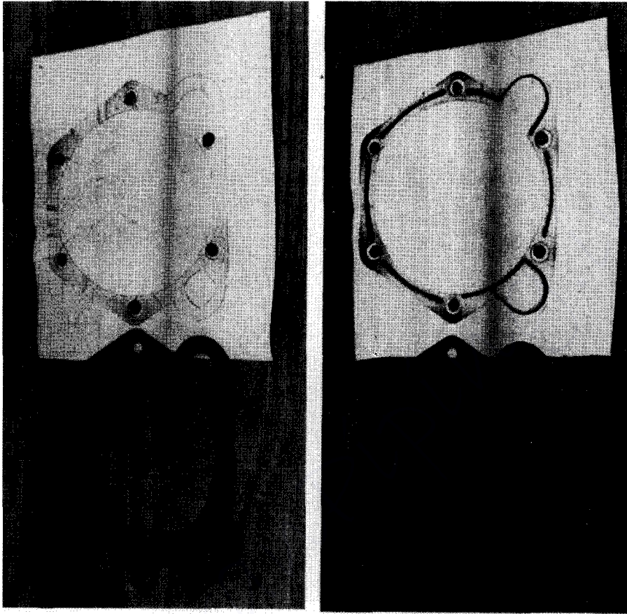
Figure 5.18 Stress impressions of gaskets with and without printed beads.
