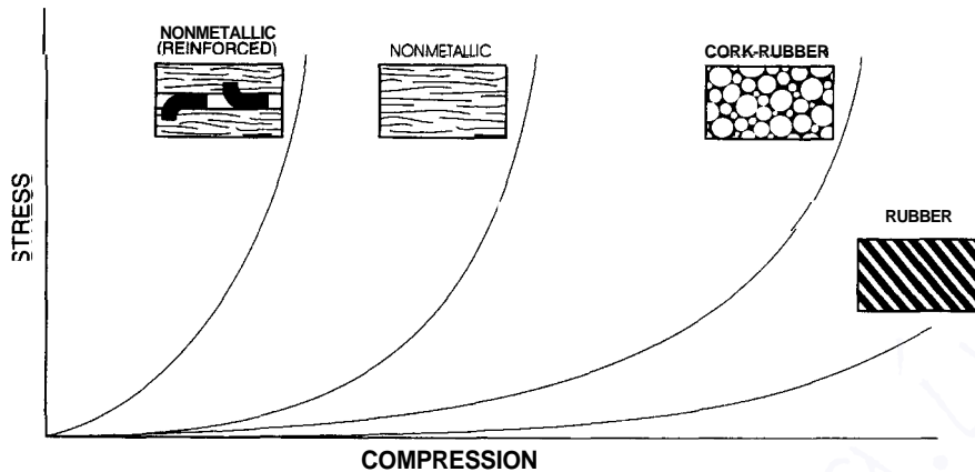
Figure 2.20 Stress versus compression for various gasket materials.
