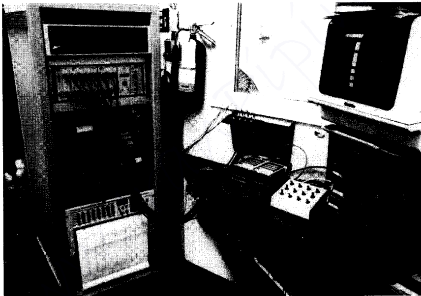
Figure 10.38 Measuring instrumentation used in gap sensor testing
