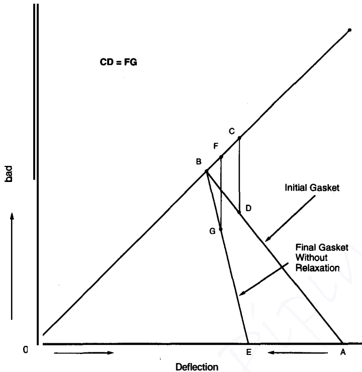
Figure 5.5 Stiffening of a gasket.
