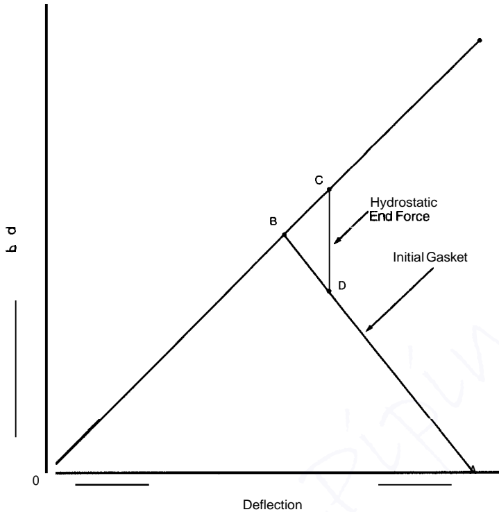
Figure 5.4 Identification of the hydrostatic end force
