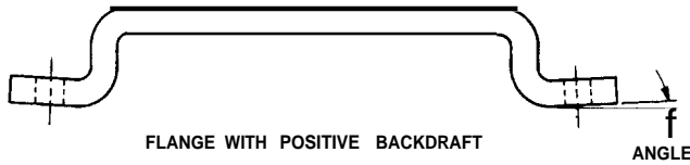
Figure 2.7 Flange with positive backdraft.
