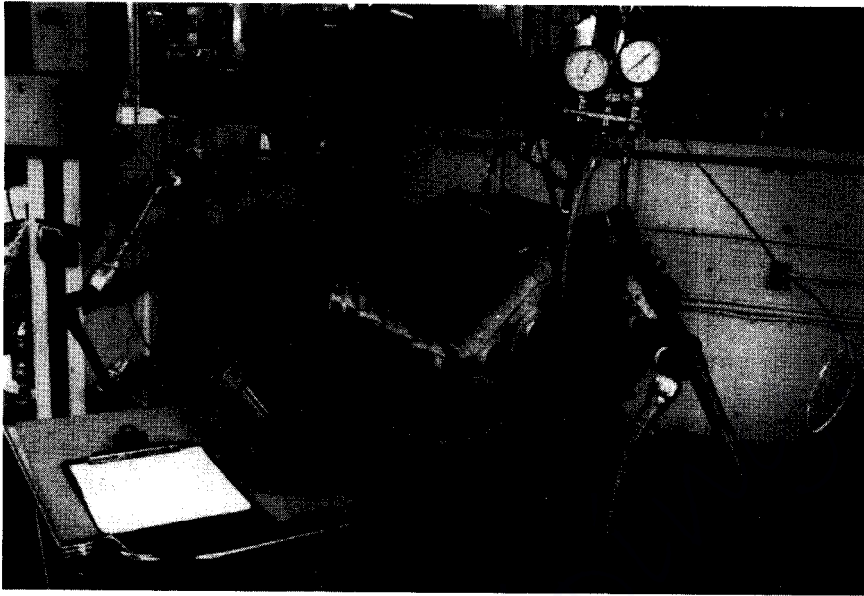
Figure 10.33 Engine being vacuum tested
