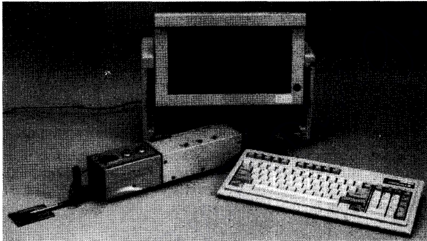
Figure 7.10 Surface finish measuring system.
