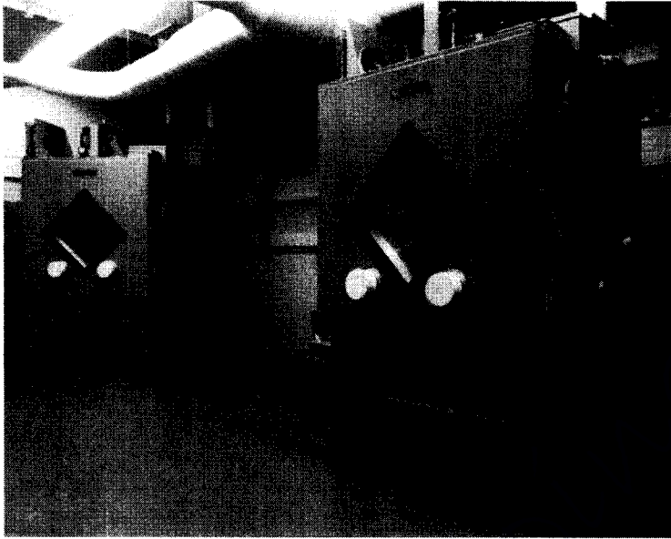
Figure 7.13 Vibration table and environmental chamber testing setup
