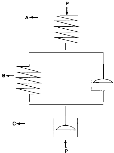
Figure 2.1 Mechanical model of a typical gasket.
