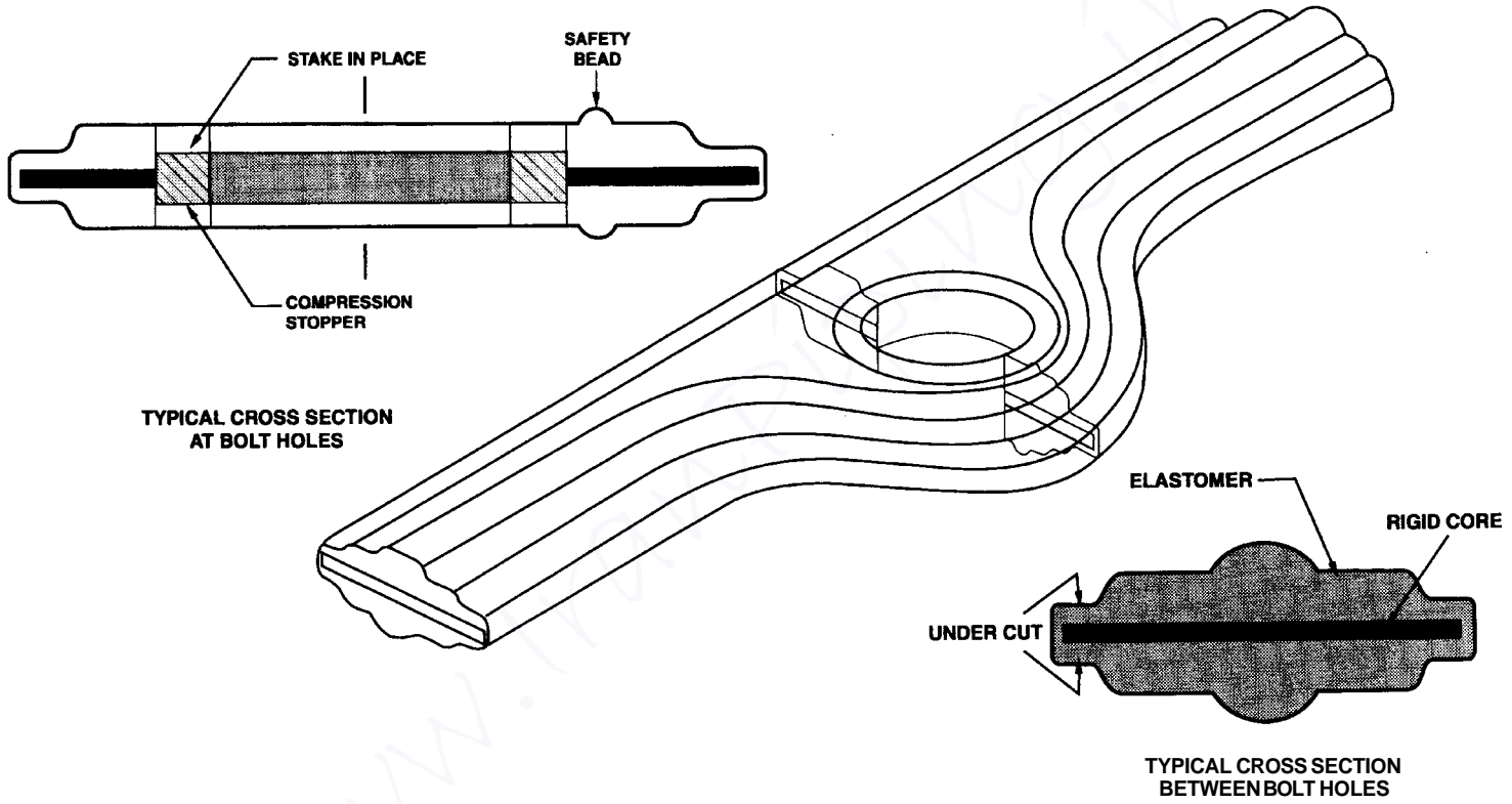
Figure 6.3 Compression limiter design.
