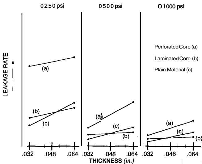
Figure 5.14 Sealability versus thickness for the various constructions.
