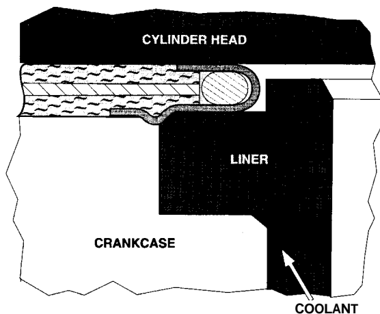
Figure 10.15 Wet liner engine.
