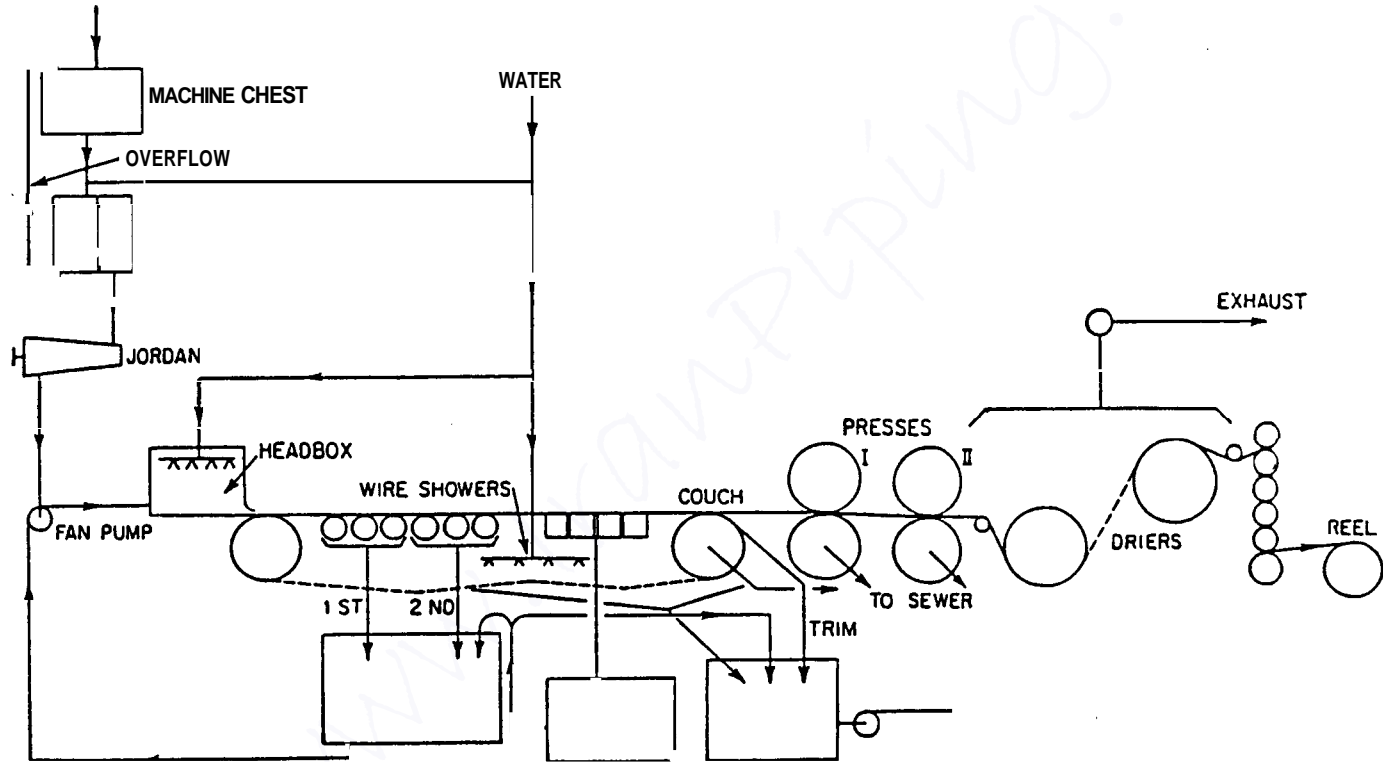
Figure 1.2 Fourdrinier process.
