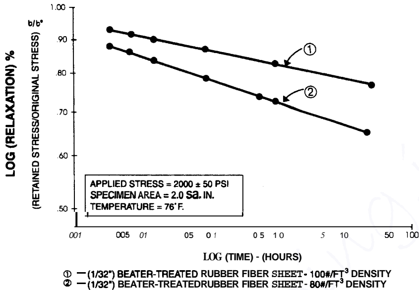
Relaxation of gasket materials; log-log plot: Effect of density
