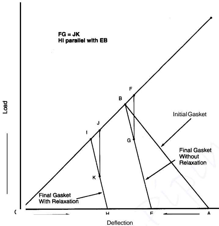
Figure 56 The effect of gasket relaxation.
