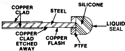
Figure 10.17 Thick steel plate gasket.
