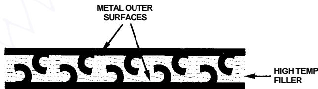
Figure 10.19 Metal-clad gasket.
