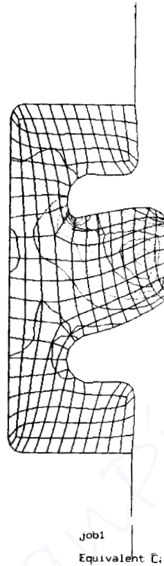
Figure 8.5 An FEA of the compressed molded bead.
