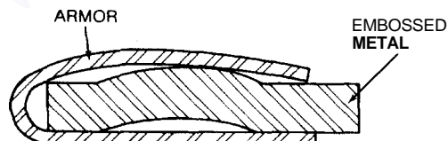
Figure 10.14 Armored embossed metal gasket.
