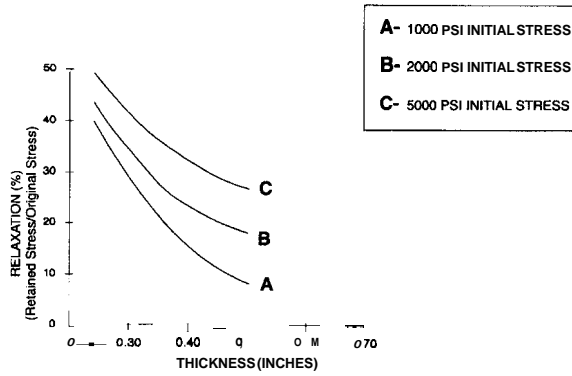
Figure 3.2 Relaxation versus gasket thickness.
