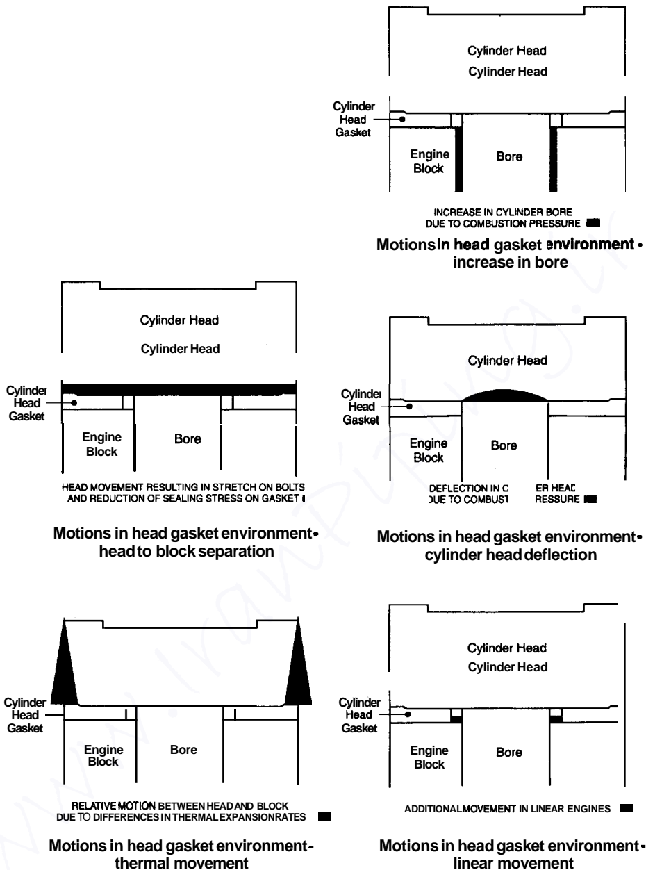
Figure 10.21 Various motions in the head gasket environment.
