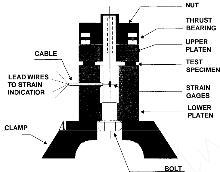
Figure 3.1 Schematic diagram of the ASTM relaxometer.
