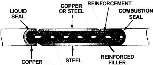
Figure 10.6 Sandwich gasket with reinforcements.
