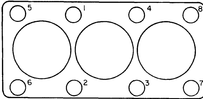
Figure 2.15 Spiral fastening sequence.
