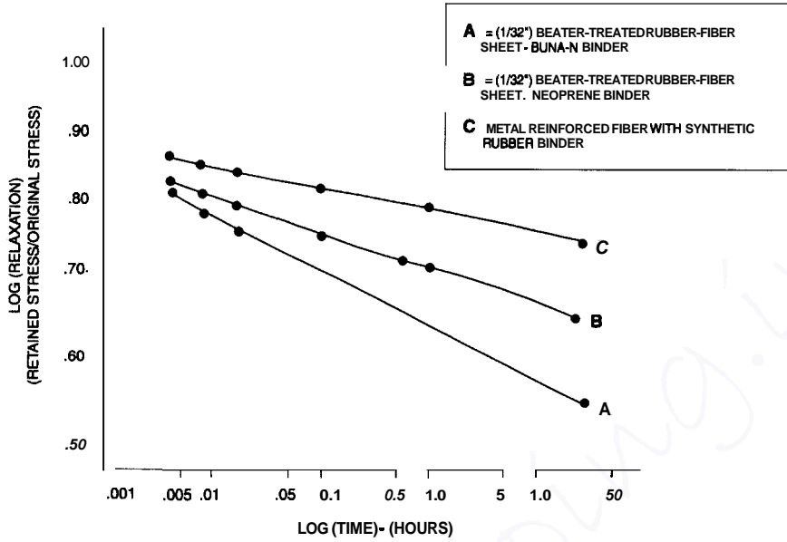
Figure 3.5 Relaxation of gasket materials, loglog plot.
