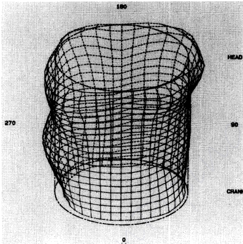
Figure 10.32 Three-dimensional plot of cylinder bore distortion.
