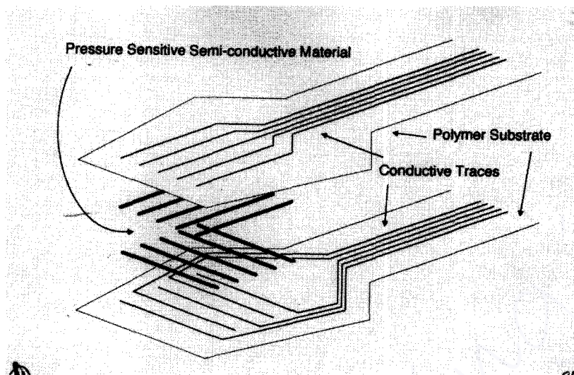
Figure 2.28 Electrical sensor construction.
