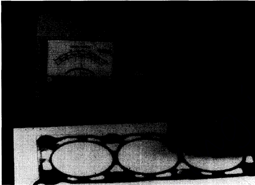
Figure 2.25 Fuji prescale film densitometer stress impression reading.
