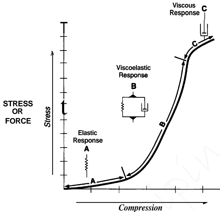
Figure 2.2 Gasket force deflection.
