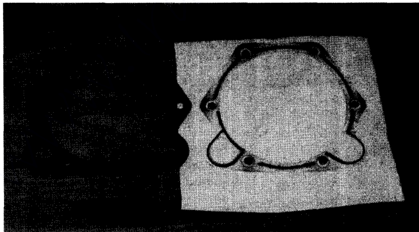
Figure 2.23 Carbonless paper stress impression of a gasket.
