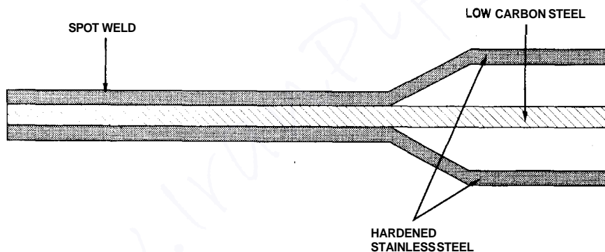
Figure 10.26 Multiple-layer embossed exhaust gasket.
