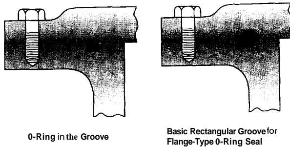
Figure 6.7 Regular and rectangular O-ring in grooves.
