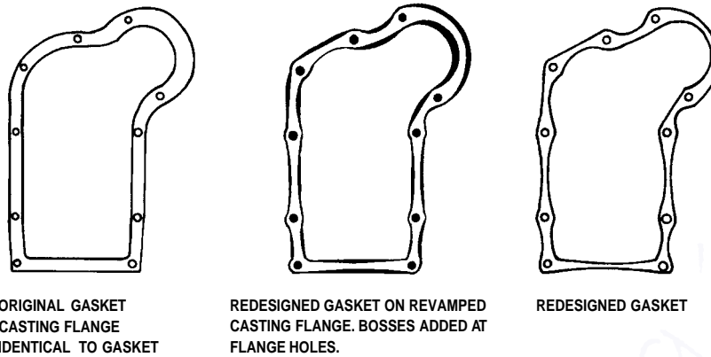
Figure 2.11 Sculptured design of gasket—original versus redesigned gasket for improved sealing.
