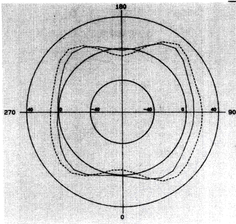
Figure 10.31 Radial plot of bore distortion
