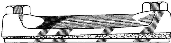
Figure 2.8 Tipping or nonparallelism in a flange
