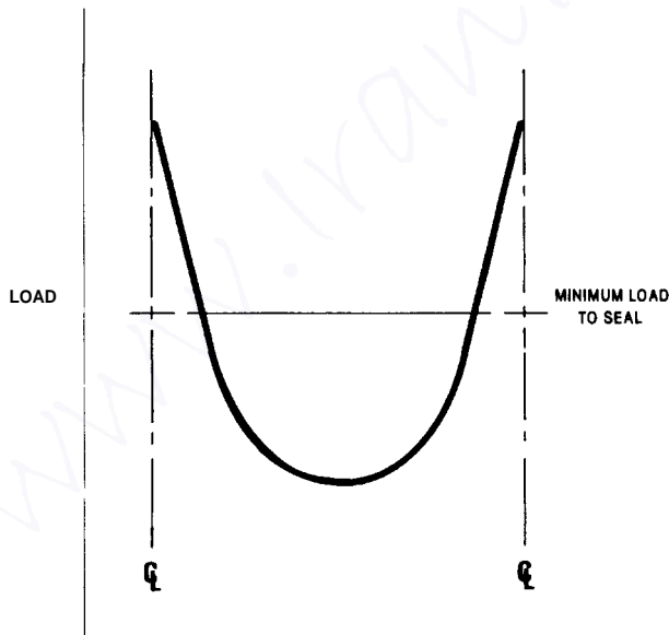
Figure 2.4 Midpoint loading between bolts.
