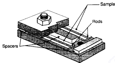
Figure 7.3 Split resistance fixture.
