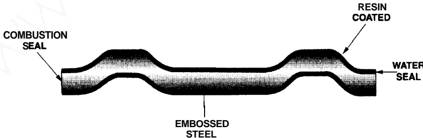
Figure 10.7 Embossed steel shim gasket.
