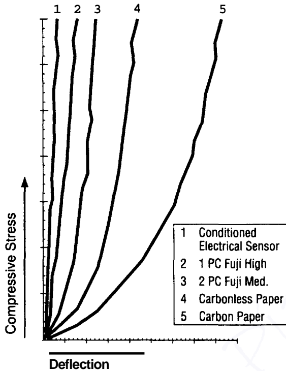
Figure 2.29 Compressive stress versus deflection for the various measurement tools.
