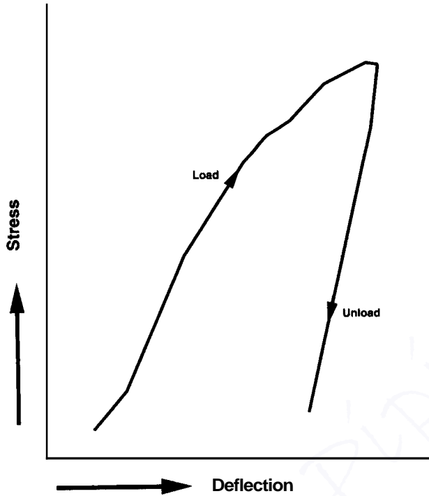
Figure 3.12 Load and unload stress versus deflection.
