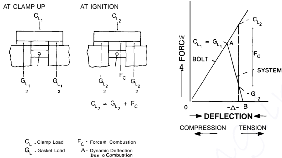
Figure 10.2 Forces and deflections in a typical head gasket joint.
