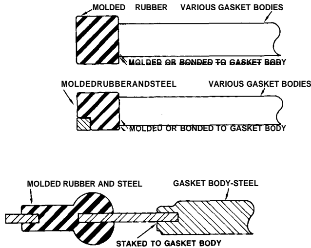
Figure 5.20 Various grommet designs.
