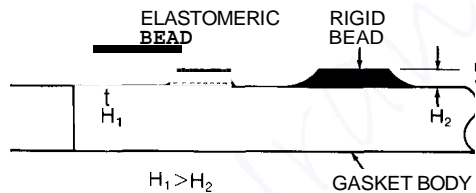
Figure 5.19 Elastomeric and rigid beads on a gasket body.
