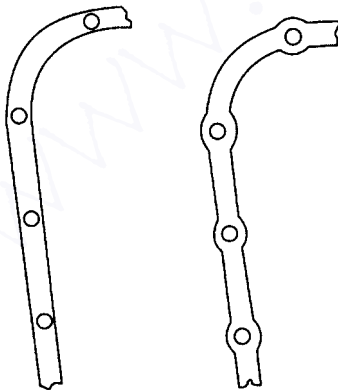
Figure 2.12 Revision to flange and gasket to prevent crush of gasket head bolt holes.
