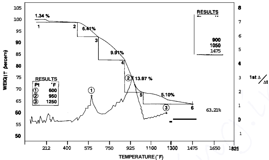
Figure 7.4 TGA plot of a nonmetallic gasket material.
