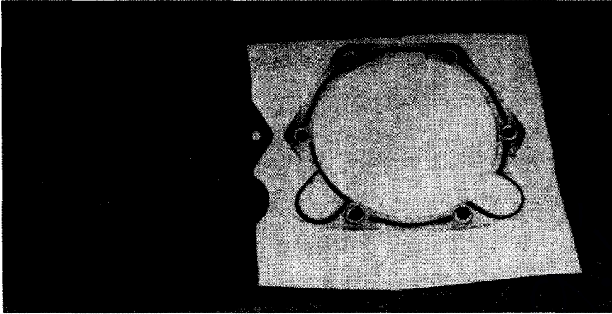
Figure 2.27 Gasket and stress distribution on it.
