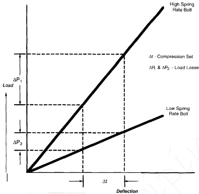
Figure 5.8 Effect of bolt spring rate on load loss.
