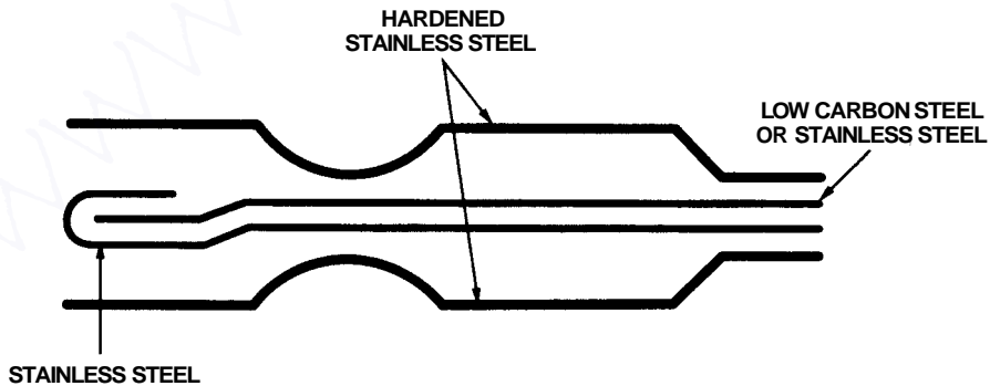
Figure 10.10 Multiple-layer steel gasket.
