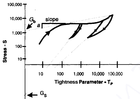
Figure 3.16 Stress versus tightness parameter in identified gasket factors or constants.
