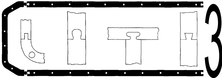
Figure 5.21 Various groove-and-tongue joints
