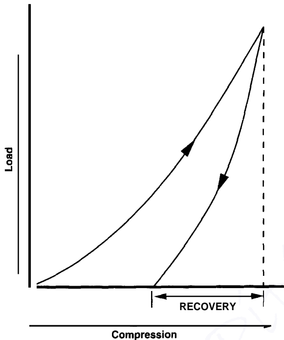
Figure 2.17 Load and unload curve for a typical non-metallic gasket material.
