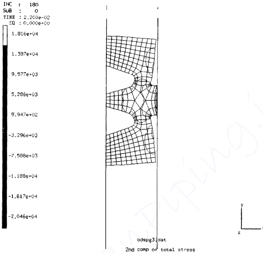
Figure 8.3 An FEA depicting a compressed gasket.
