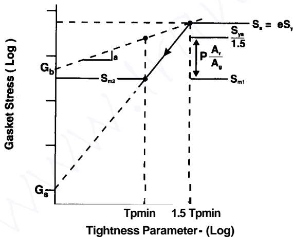
Figure 3.17 Stress versus tightness and seating identification.
