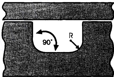
Figure 6.6 O-ring groove.
