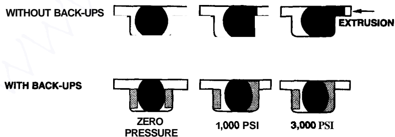
Figure 6.13 O-ring configuration with and without backup rings.
