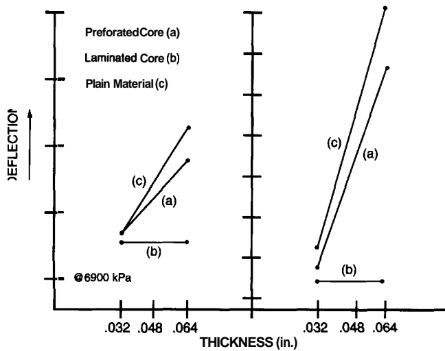
Figure 5.13 Compressive deflection versus thickness of various constructions or composites.
