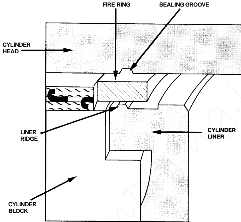
Figure 10.16 Ridge and groove gasket.
