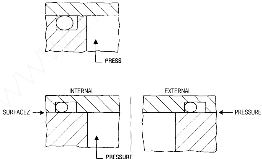
Figure 6.9 O-ring seal axial gland designs.
