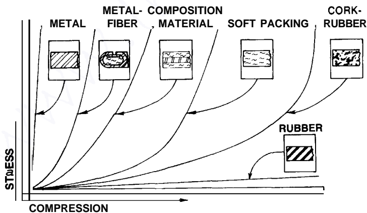
Figure 2.16 Stress versus compression for various gasket materials
