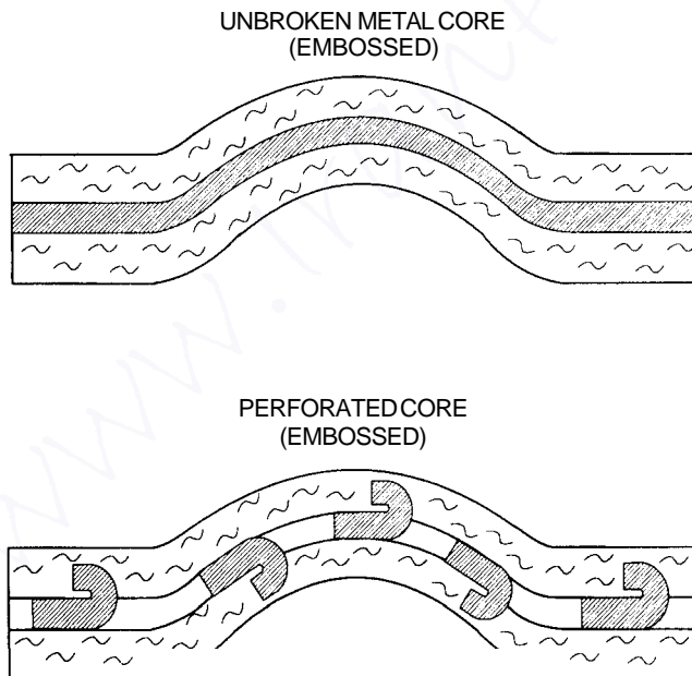
Figure 5.15 Unbroken and perforated metal core emboss.
