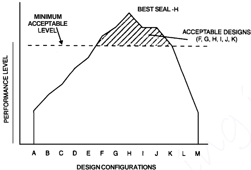
Figure 10.3 Performance level for various gasket designs.
