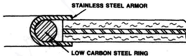
Figure 10.13 Wire ring gasket.
