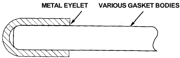
Figure 5.10 Eyeletted gasket.
