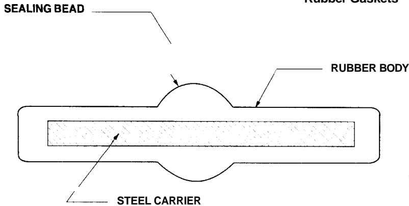
Figure 6.2 Metal core supported molded rubber gasket.
