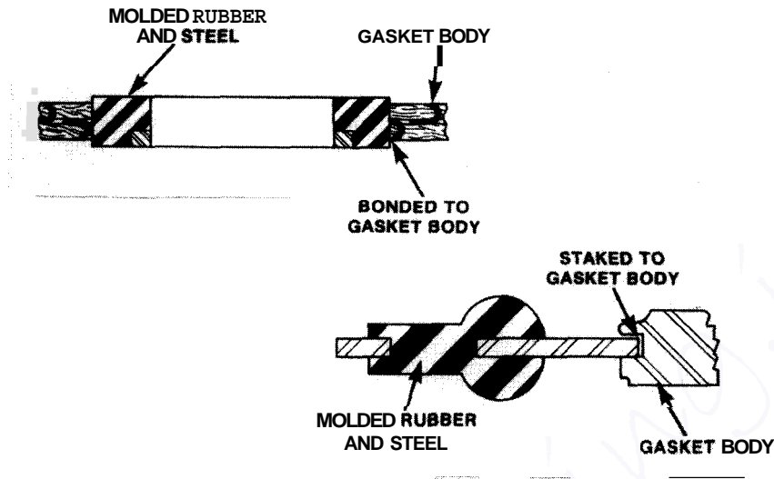
Figure 10.22 Molded rubber grommets used in head gaskets.
