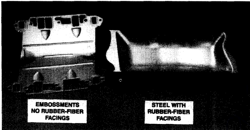
Figure 10.23 Intake manifold gasket with combined oil splash plate
