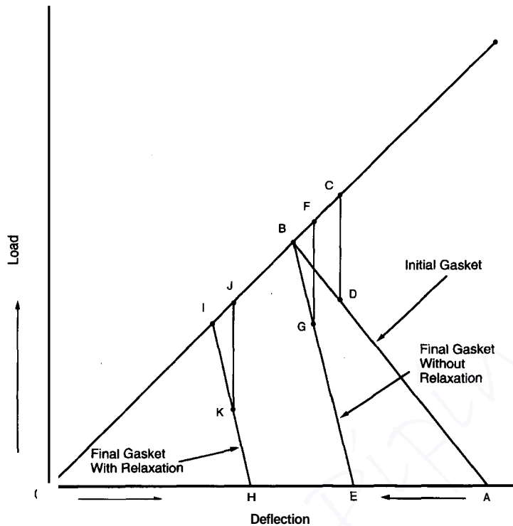
Figure 5.7 Complete gasket and joint diagram.
