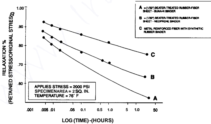
Figure 3.6 Relaxation of gasket materials, semilog plot.
