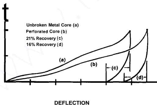
Figure 5.16 Load deflection and recovery.
