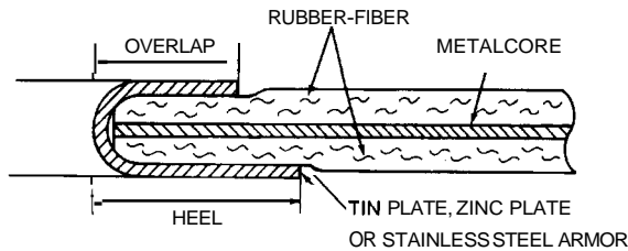
Figure 10.11 Armored gasket.
