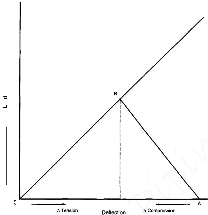
Figure 5.3 Gasket and joint diagram.
