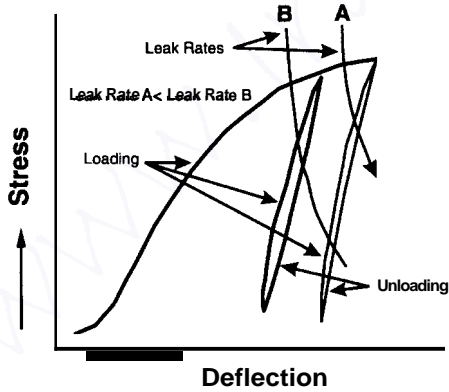
Figure 3.13 Stress versus deflection and leak rates.
