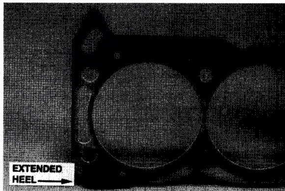
Figure 10.12 Extended heel.
