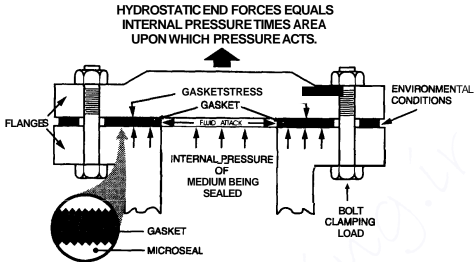
Figure 1.1 Nomenclature of a gasketed joint.
