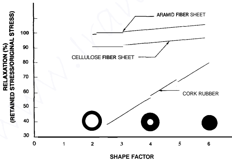
Figure 3.9 Relaxation versus the shape factor.
