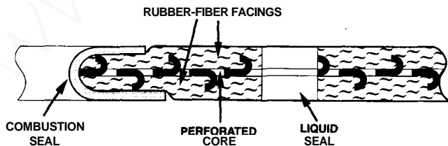
Figure 10.8 Perforated core head gasket.
