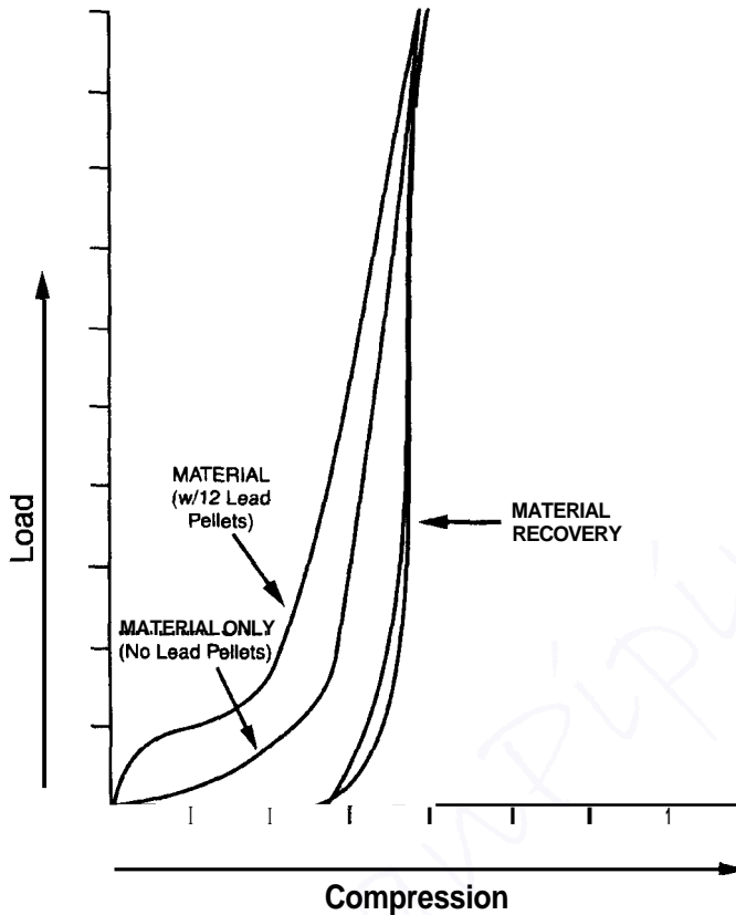
Figure 2.21 Load versus compression for gasket with and without lead pellets.
