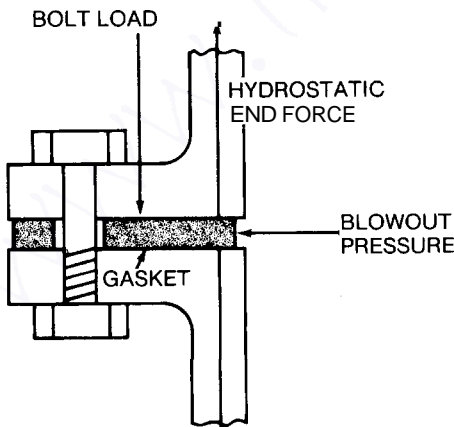
Figure 2.9 Blowout pressure in a gasketed joint.
