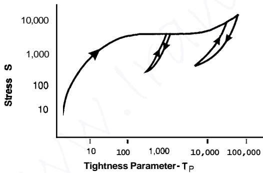
Figure 3.15 Stress versus tightness parameter.
