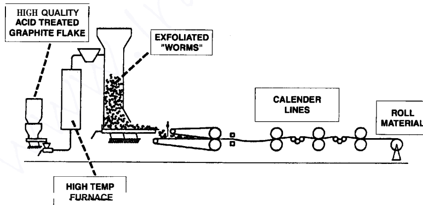
Figure 1.5 Expanded graphite process.
