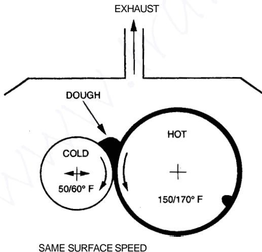
Figure 1.4 Compressed material process.
