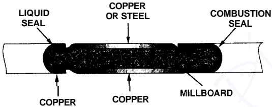
Figure 10.5 Sandwich gasket.
