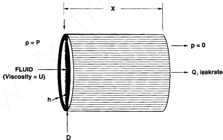
Figure 9.1 Fluid dynamics leakage rate.
