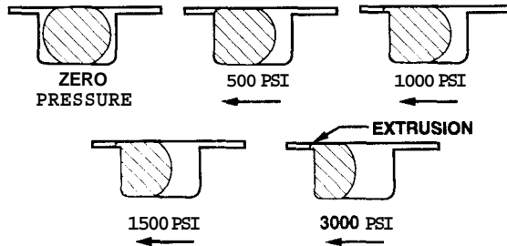
Figure 6.12 O-ring configuration under varying internal pressures.
