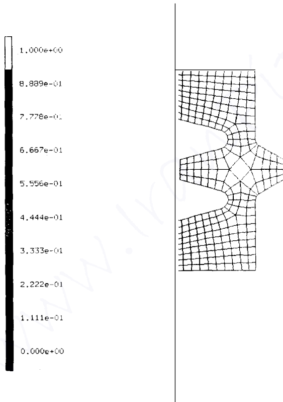
Figure 8.2 An FEA depicting an uncompressed gasket.
