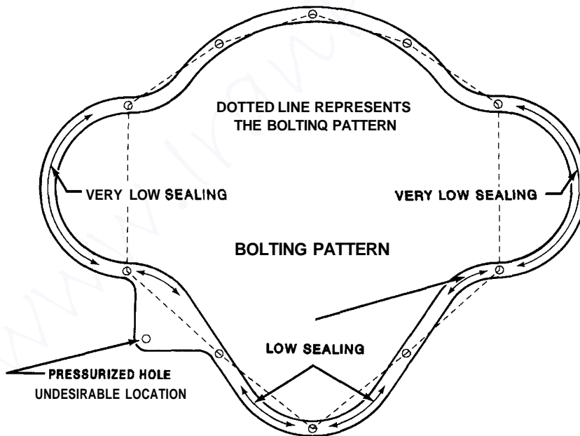
Figure 2.10 Good and poor sealing locations.
