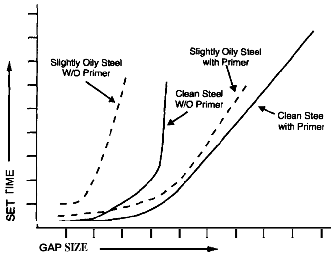
Figure 9.5 Set time versus gap size for an anaerobic material.
