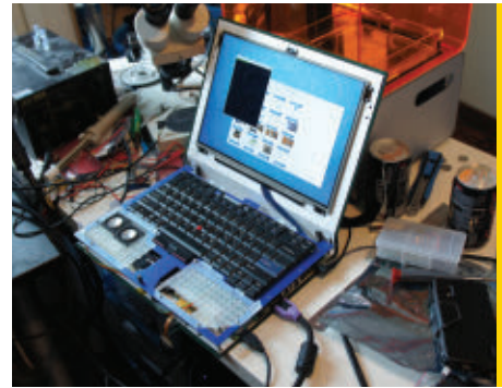
A DIY laptop parked in front of the Form 1 3D printer used to make its body panels.
