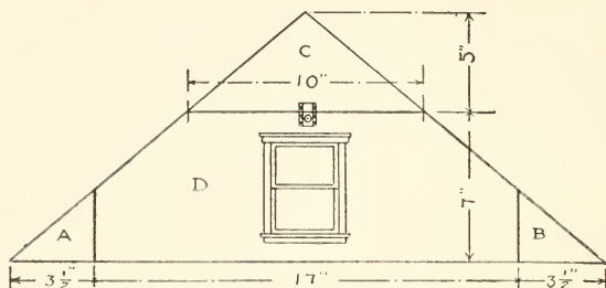
FIG. 240. — Front Gable-End.
