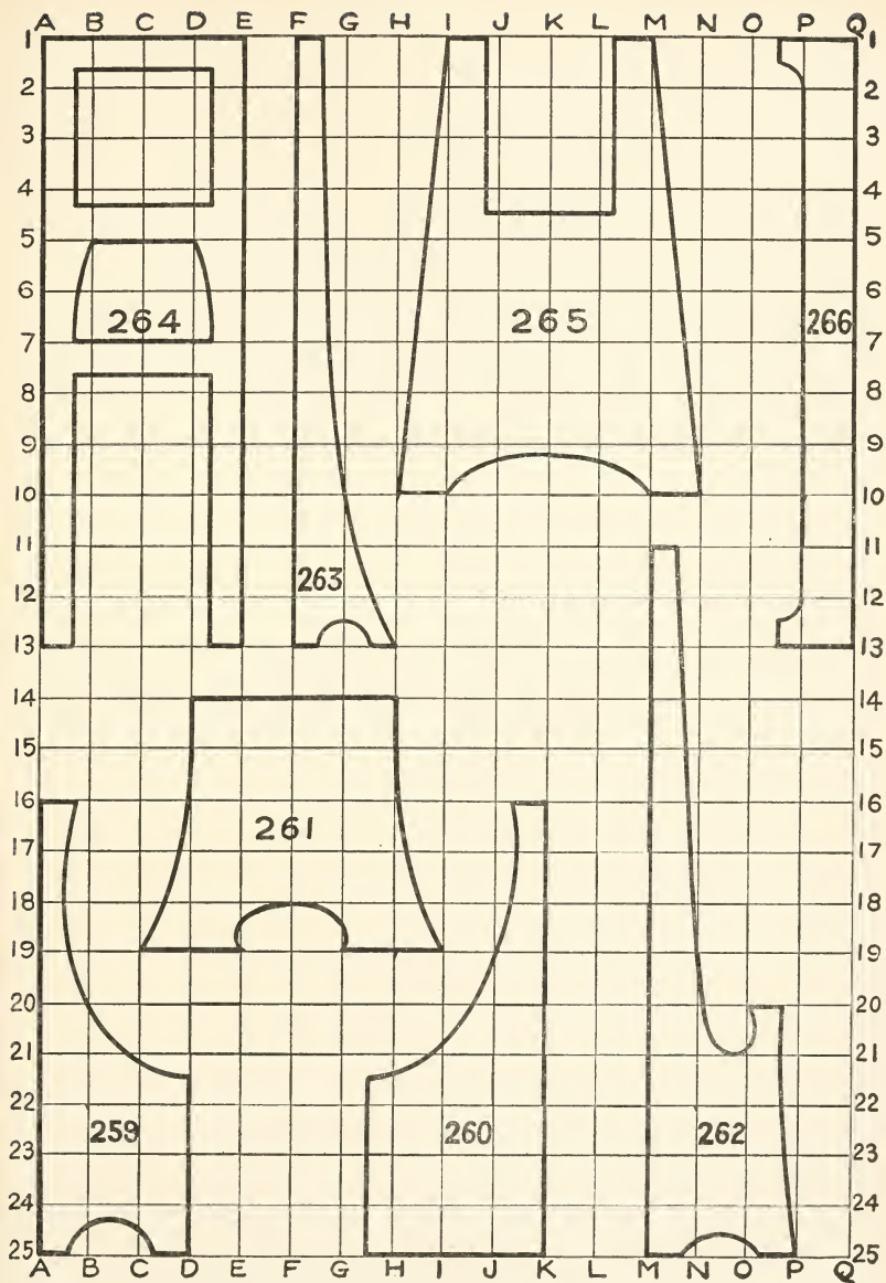
FIGS. 259-266. — Patterns for Furniture.
