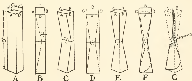
FIG. 44.—How to Prepare a 9-inch Propeller.
