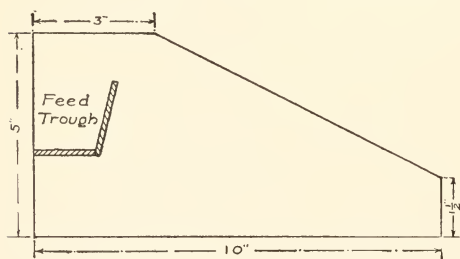
FIG. 241. — Stall Partitions.
