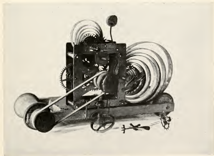
FIG 161. THE FRAMEWORK.
