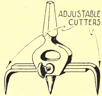
FIG 3 DISC CUTTER
