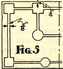
HALF PLAN OF PIERCED BOTTOM
