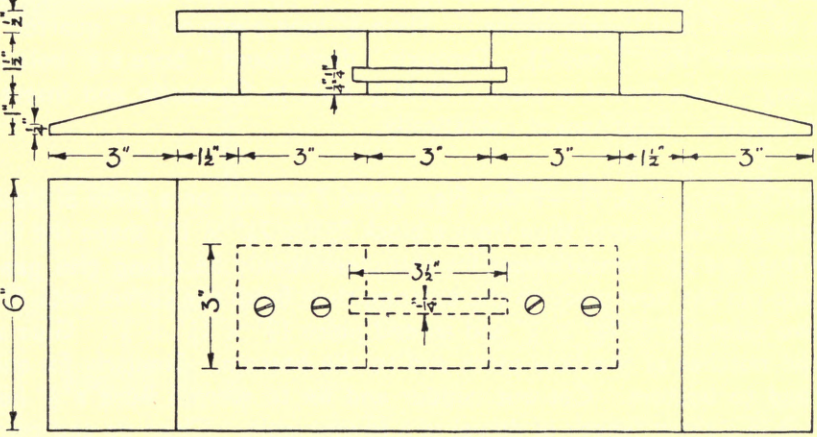
SECTION THROUGH CENTRE OF STATION
