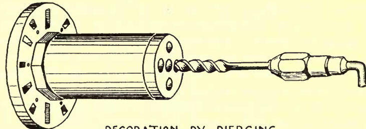
FIG 3 DECORATION BY PIERCING BLOCK MOUNTED ON FACE PLATE
