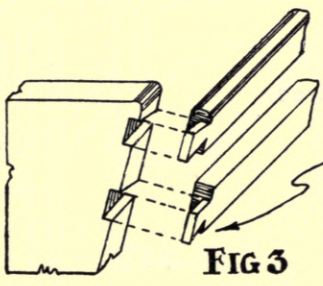
JOINTS OF RAIL WITH HEAD & FOOT AND OF HEAD & FOOT WITH BOTTOM
