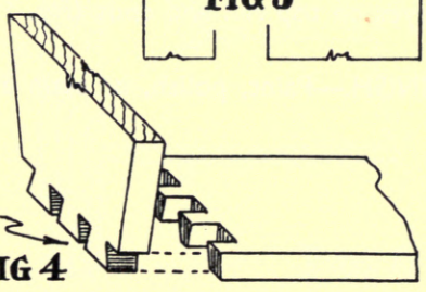
JOINTS OF RAIL WITH HEAD & FOOT AND OF HEAD & FOOT WITH BOTTOM
