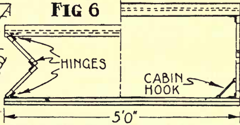
JOINT "A"
