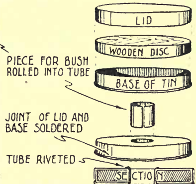
FIG 5 ASSEMBLY OF WHEEL
