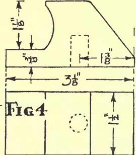
FIG 4 CENTRE OF TURRET
