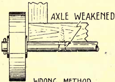
FIG 4 WRONG METHOD SCREW THROUGH AXLE
