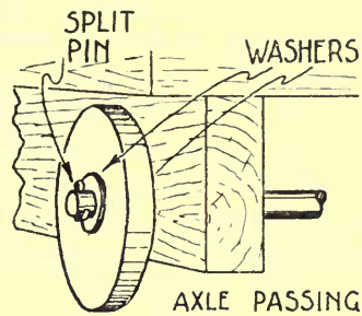
FIG 3 THROUGH BEARER
