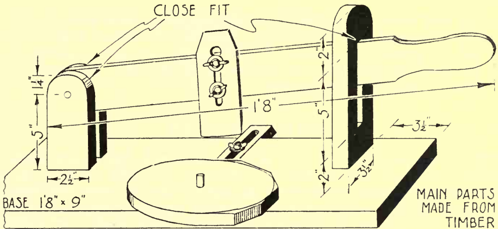
FIG 1 GUILLOTINE WITH DISC PARTLY SHAPED
