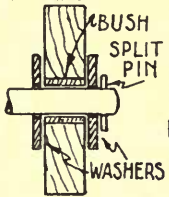
SECTION OF WHEEL
