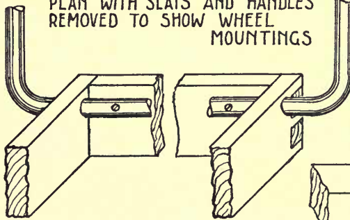
FIG 2 HANDLES SCREWED TO SIDES OF BASE
