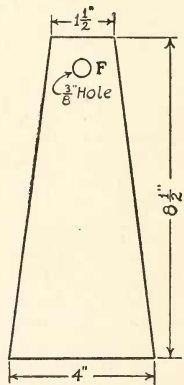
FIG. 75. — Upright.
