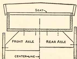
FIG. 286. — Cross-Section of the Express-Wagon.
