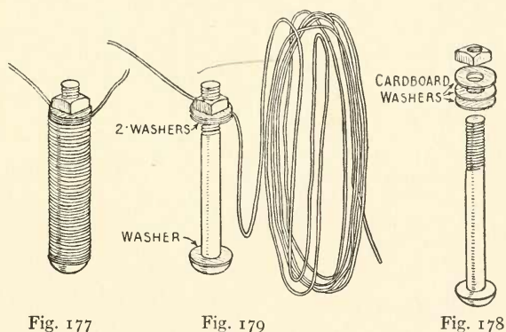
FIGS. 177-179. — The Electro-Magnet.
