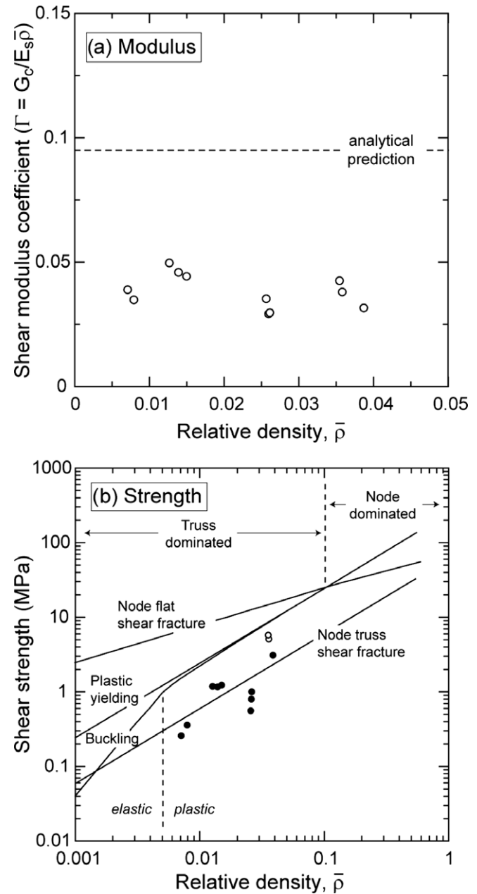
Fig. 10. Analytical predictions and experimental data for (a) the non-dimensional shear stiffness and (b) the shear strength as a function of relative density. Solid circles (●) indicate samples that failed at the nodes prior to the full peak strength.
