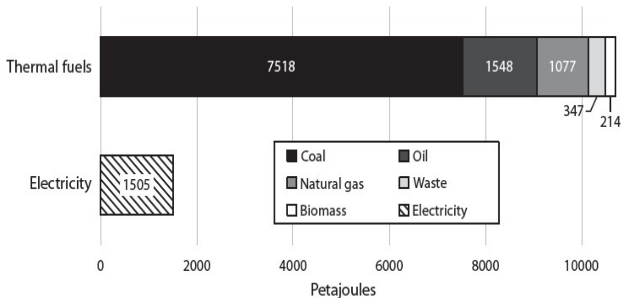
FIGURE 3.3 Global Cement Industry Energy Use in 2019 Thermal fuels are used to heat the kiln and precalciner, while most electricity is used to grind input materials and cement.
