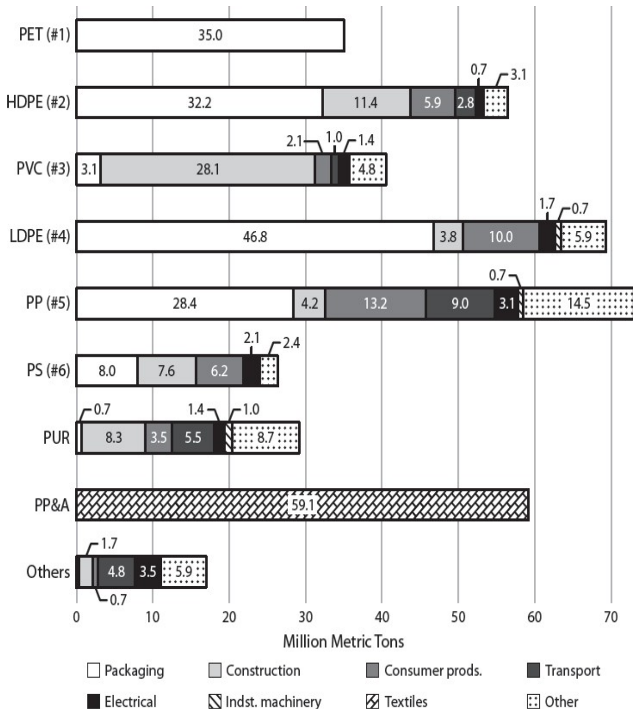
FIGURE 5.6 Global Plastic Production by Resin Type and End Use in 2015 The designations #1–6 indicate each plastic’s resin identification code, which may appear inside a triangle or “chasing arrows” symbol on rigid plastic items. PET = polyethylene terephthalate; HDPE = high-density polyethylene; PVC = polyvinyl chloride; LDPE = low-density polyethylene; PP = polypropylene; PS = polystyrene; PUR = polyurethane; PP&A = polyester, polyamide, and acrylic. “Others” includes polycarbonate (PC), acrylonitrile butadiene styrene (ABS), polymethyl methacrylate (PMMA),
