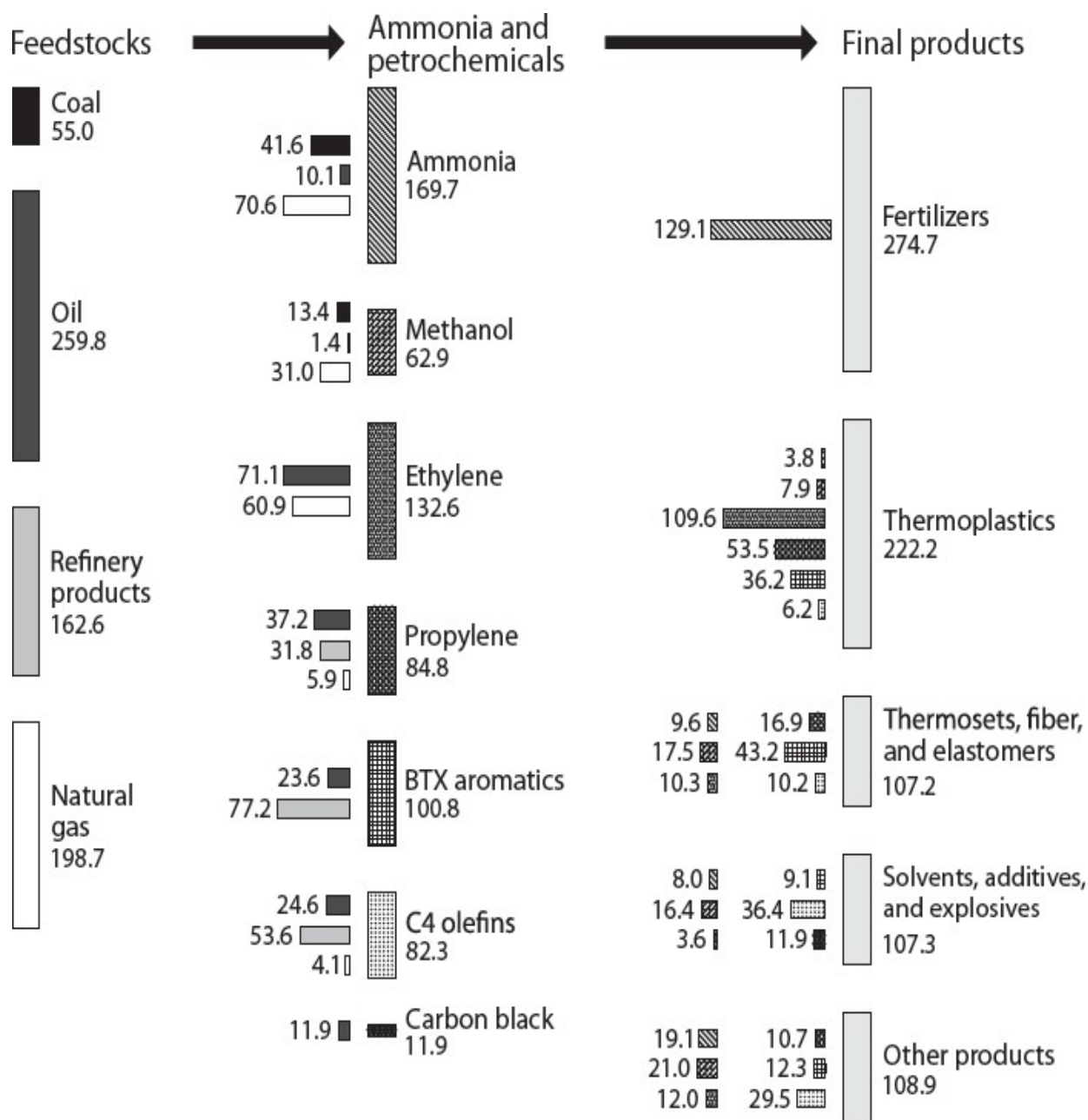
FIGURE 2.2 Material Flow from Fossil Fuel Feedstocks to Ammonia and Petrochemicals and to Final Products in 2013 Secondary reactants and secondary products are not shown (and are the reason feedstock flows do not sum to the total mass of ammonia and petrochemicals, and their flows do not sum to the total mass of final products). On-purpose technologies, which convert small amounts of natural gas, methanol, ethylene, and C4 olefins into propylene and ethylene, are not shown. Values are in millions of metric tons.
