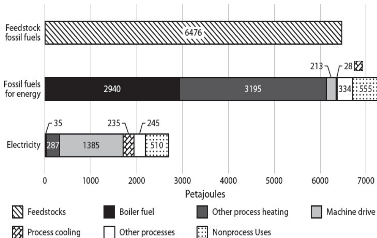
FIGURE 6.1 Uses of Fossil Fuels and Electricity by U.S. Industry in 2018 “Machine drive” includes pumps, conveyor belts, fans, robots, and other moving elements of production processes. “Other processes” includes electrochemistry and miscellaneous processes. “Nonprocess uses” include heating, cooling, and lighting buildings for the comfort of workers, using vehicles to transport items around an industrial site, and the like. The figure excludes energy whose fuel type and end use were not reported (including biomass and waste, refinery fuel gas, blast furnace gas, and steam purchased from external suppliers, such as district heating plants).
