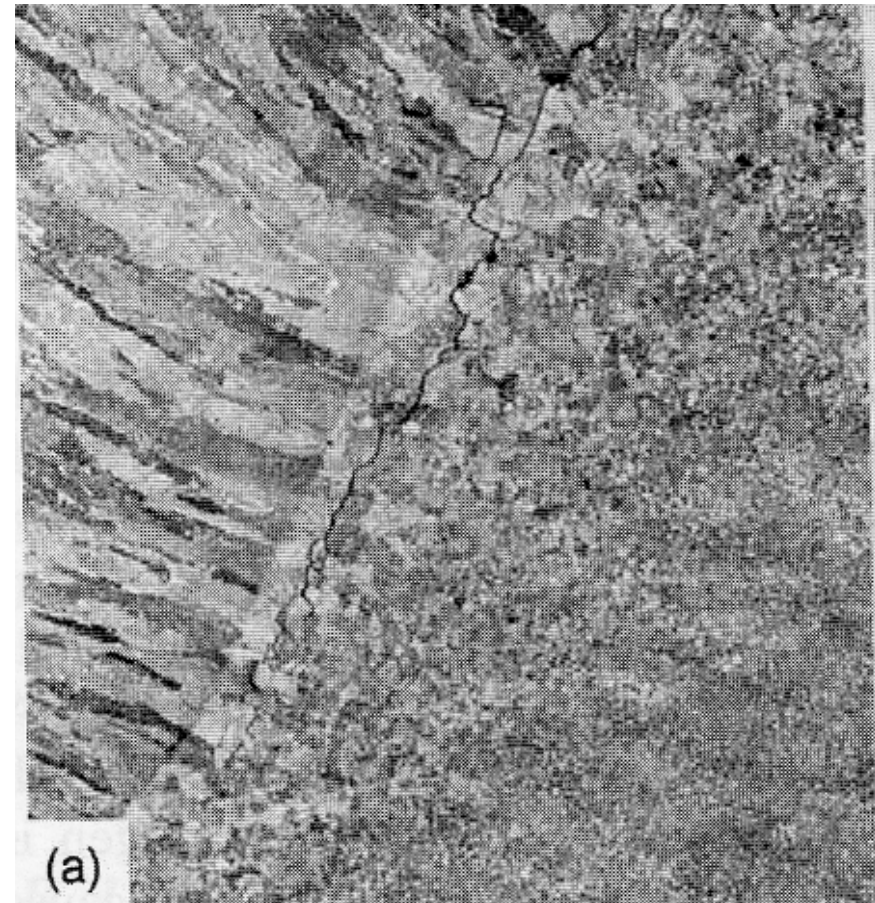
Reheat Cracking
