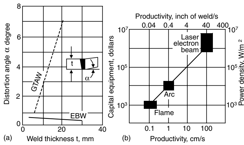
Figure 1.3 Comparisons between welding processes: (a) angular distortion; (b) capital equipment cost. Reprinted from Mendez and Eagar (2).
