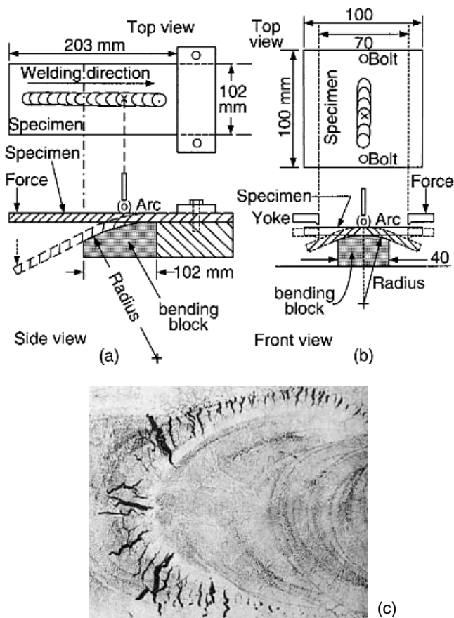
Figure 11.6 Solidification cracking tests: (a) Varestraint (15); (b) transverse Varestraint (16); (c) cracking in a ferritic stainless steel Varestraint specimen (17). (c) Reprinted from Krysiak et al. (17), courtesy of ASM International.
