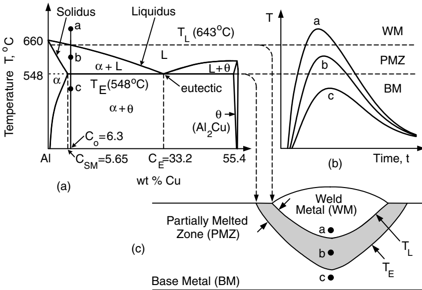
Figure 12.3 Formation of PMZ in 2219 aluminum weld: (a) Al-rich side of Al-Cu phase diagram; (b) thermal cycles; (c) transverse cross section.
