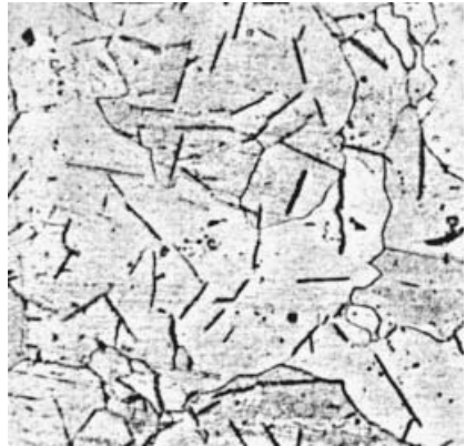
Figure 3.6 Iron nitride in a ferrite matrix ( \times 500 ). From Seferian (15).
