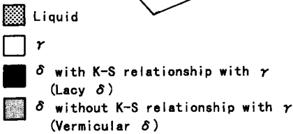
Figure 9.6 Mechanism for the formation of vermicular and lathy ferrite. Reprinted from Inoue et al. (11).
