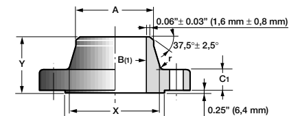
WELDING NECK
