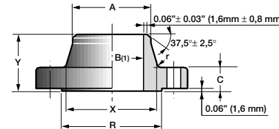
WELDING NECK
