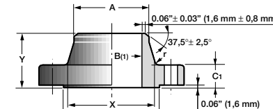
WELDING NECK
