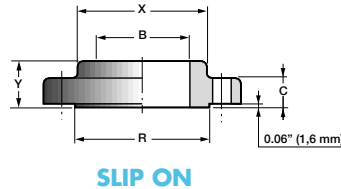
SLIP ON
