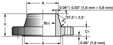
WELDING NECK
