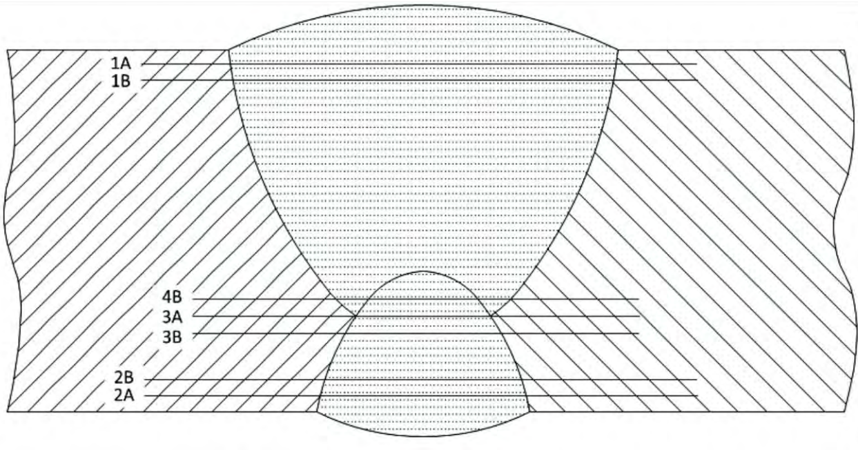
Figure C.2 — Rows of indentations in butt welds from two sides
