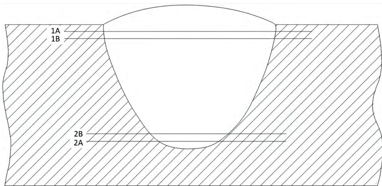
Figure C.3 — Rows of indentations in partial penetration butt welds
