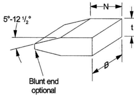
Figure 11(b): DCB Specimen—Double-Tapered Wedge
