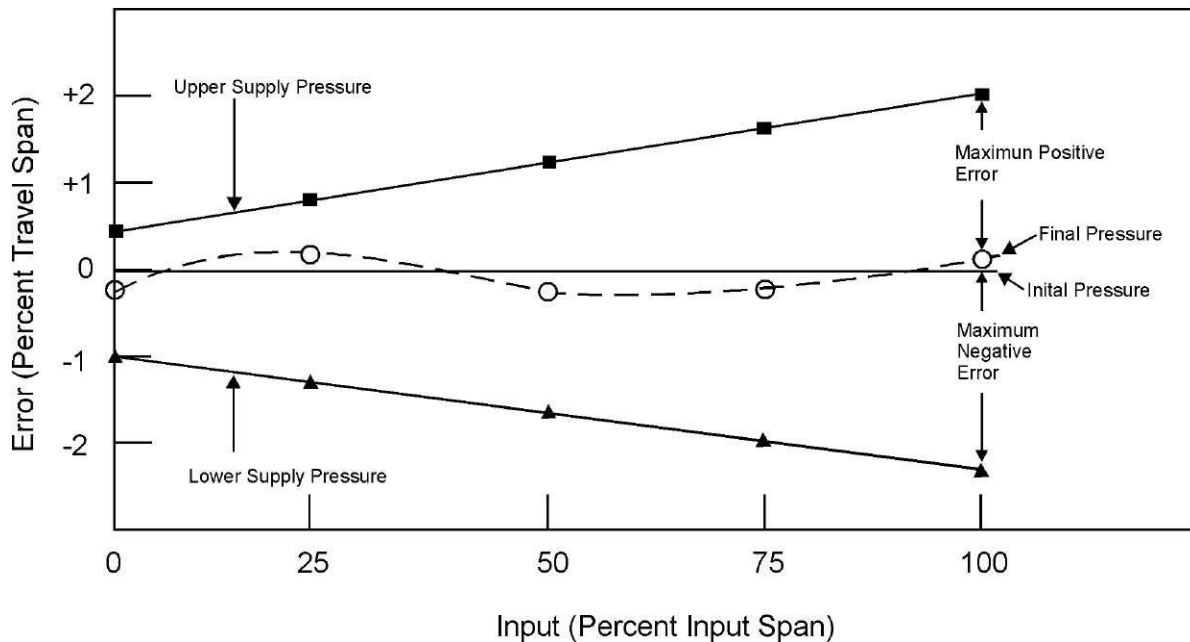
Figure 2 — Supply pressure influence
