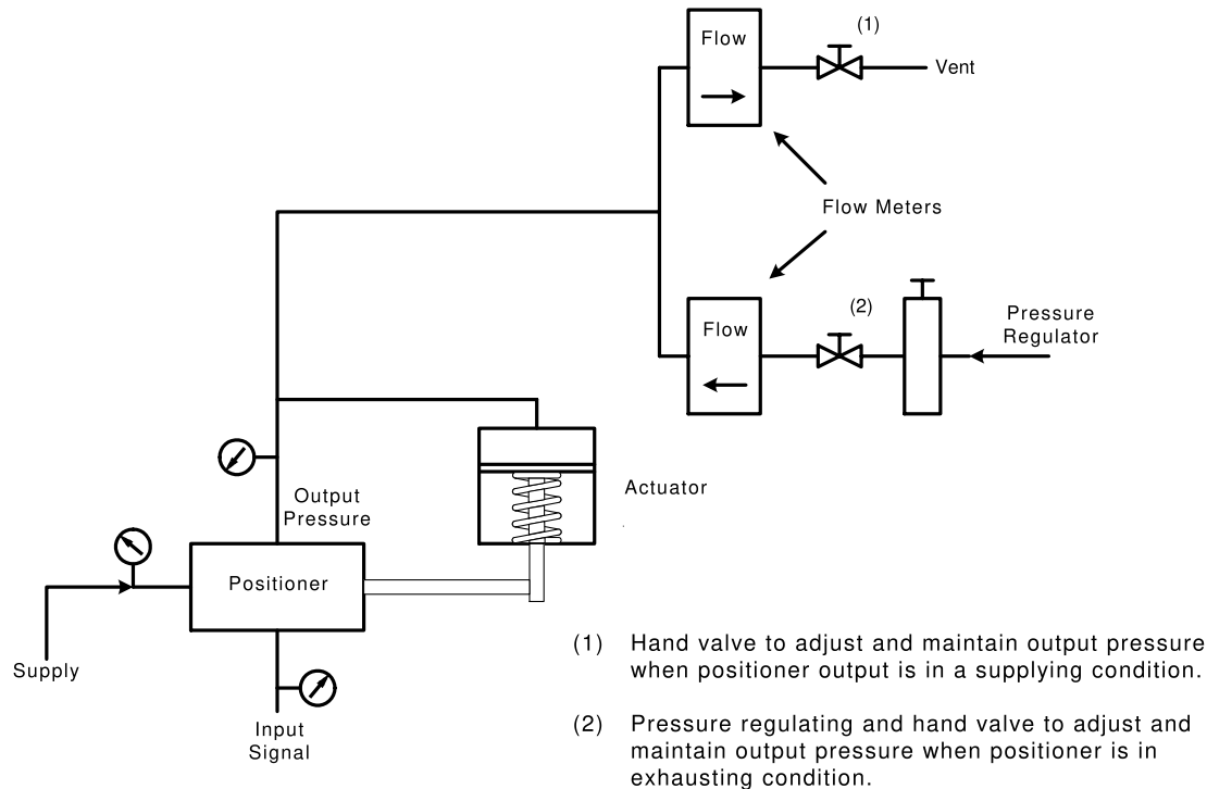
Figure 8 — Typical schematic for flow capacity tests
