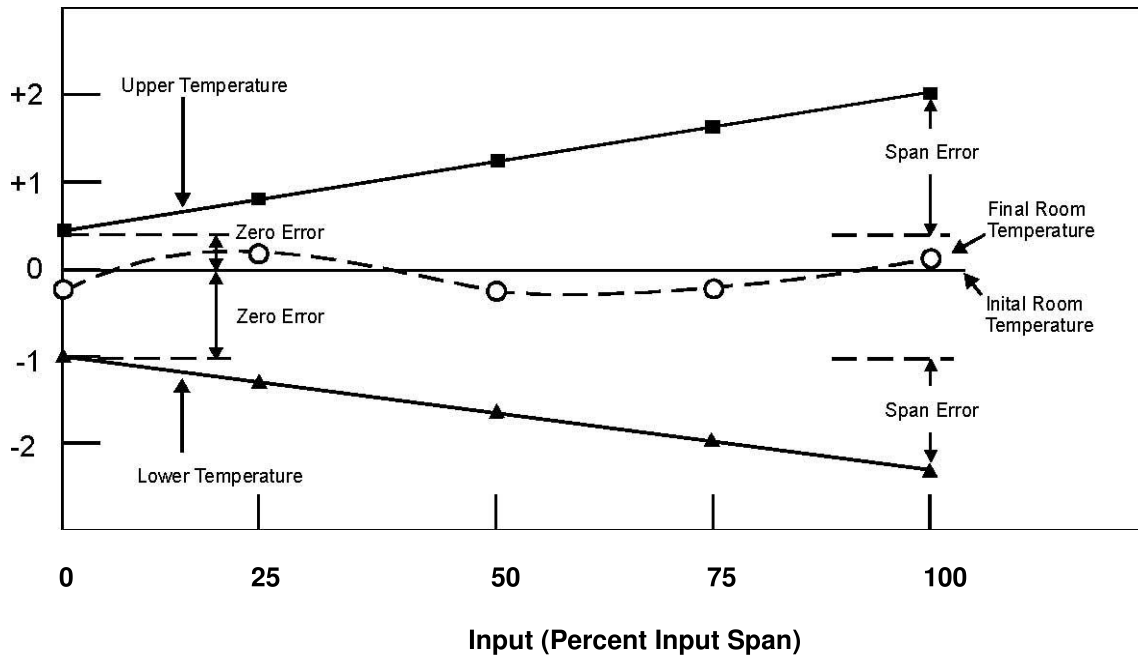
Figure 3 — Ambient temperature influence
