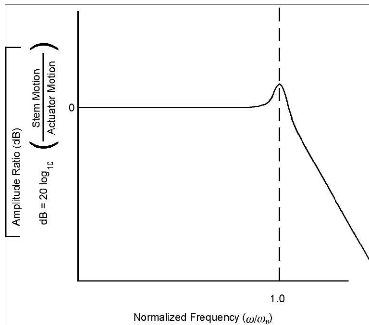
Figure 4 — Relative stem motion for typical linear actuator
