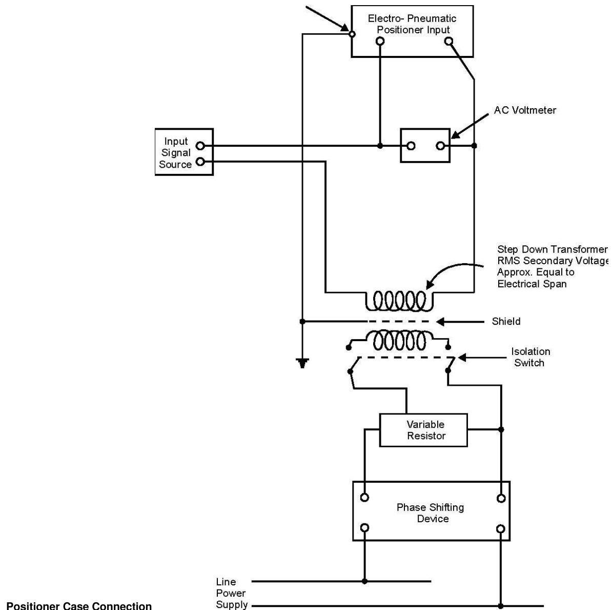
Figure 6 — Test circuit for normal mode interference influence
