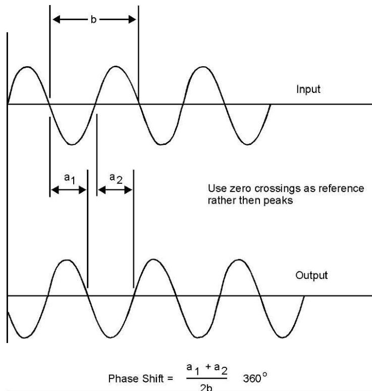
Figure 17 — Determination of phase shift for distorted output
