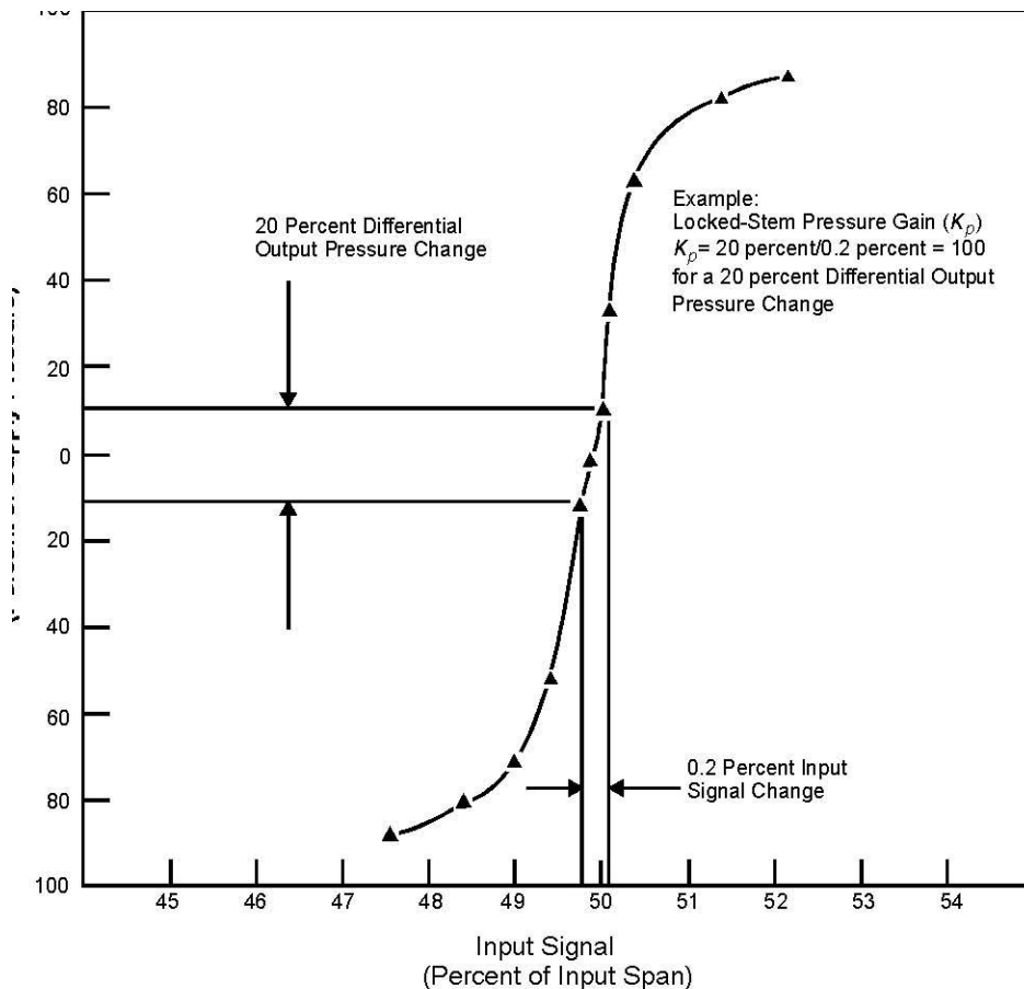
Figure 11 — Locked-stem pressure gain (double-acting)
