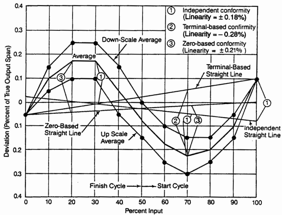
Figure 1 — Calibration curve (of data from Table 1)
