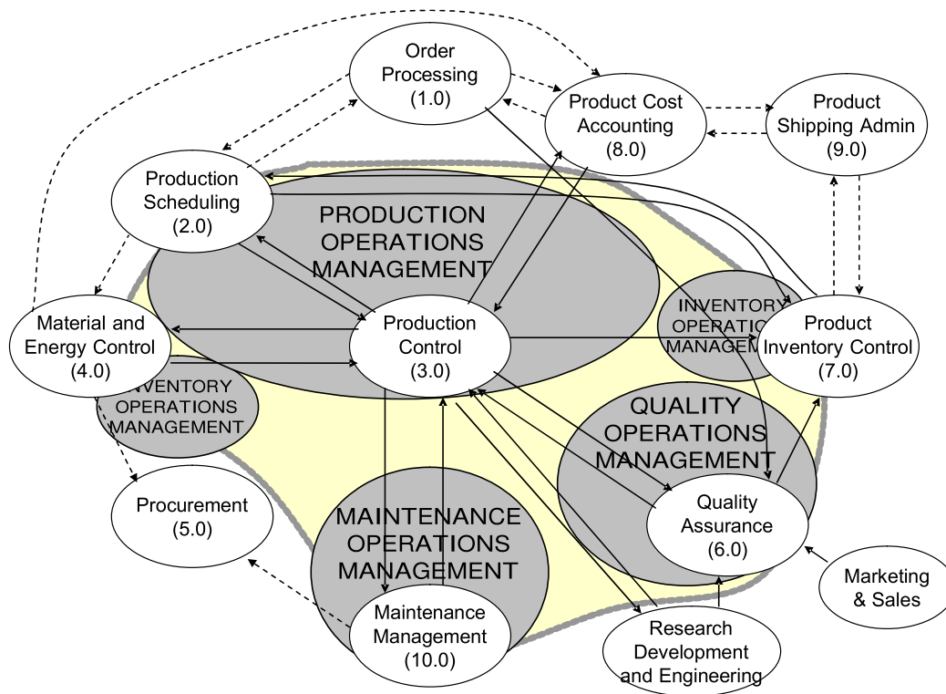
Get more FREE standards from Standard Sharing Group and our chats Figure 8 – Manufacturing operations management model
