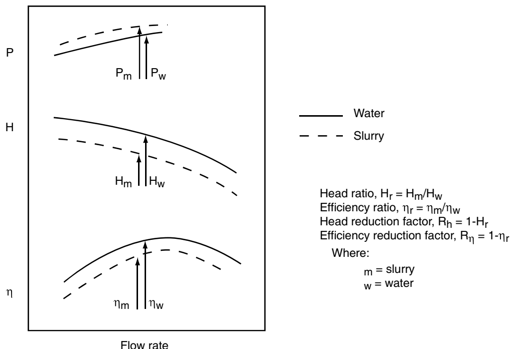
Figure 12.19 — Effect of slurry on pump characteristics (schematic)
