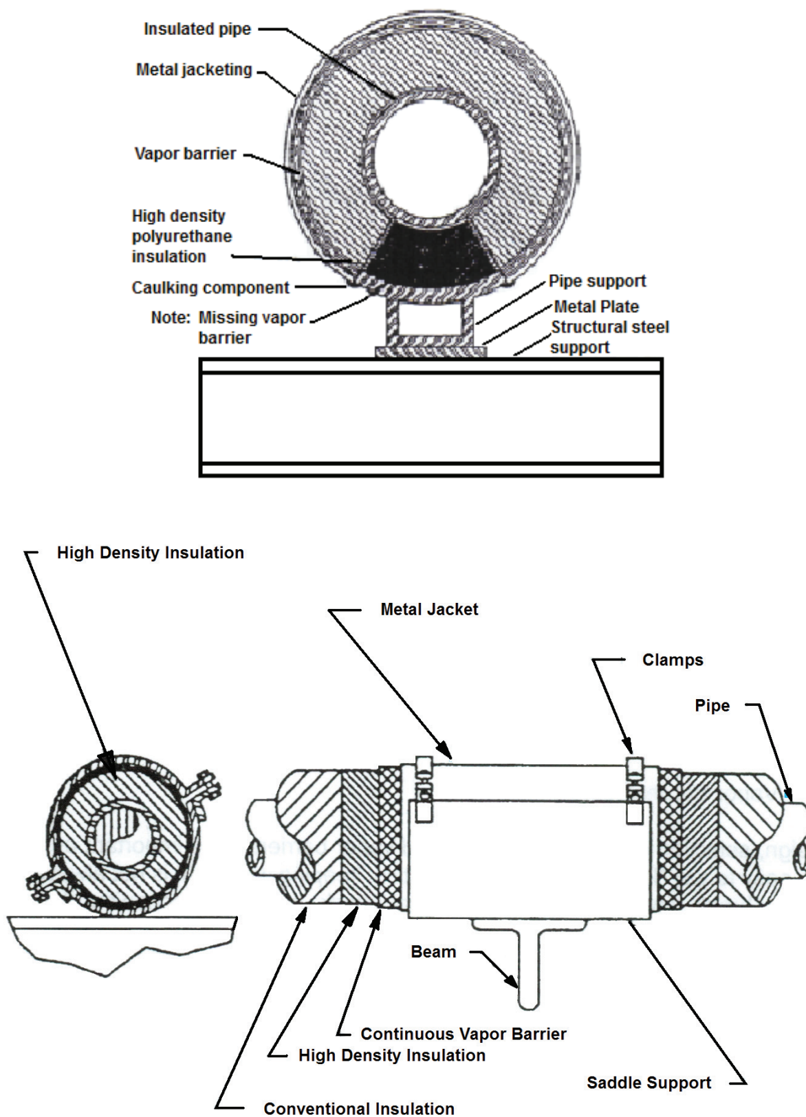
Figure B.3—Method for Insulating Pipe Support with and Without Continuous Vapor Barrier
