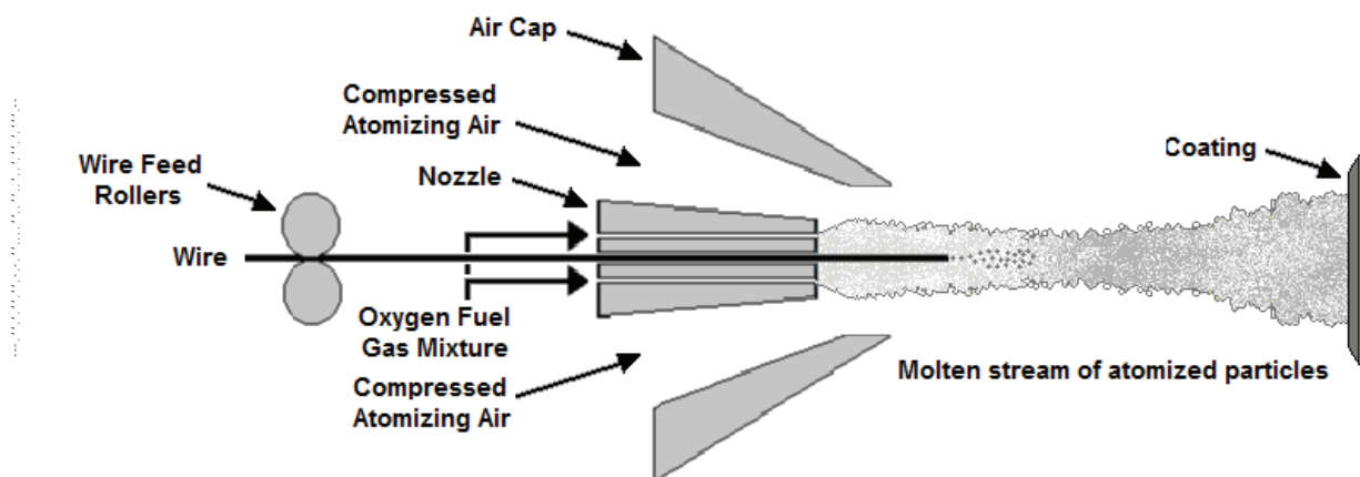
Figure 24—Schematic of Oxy-fuel Wire Spray Processes
