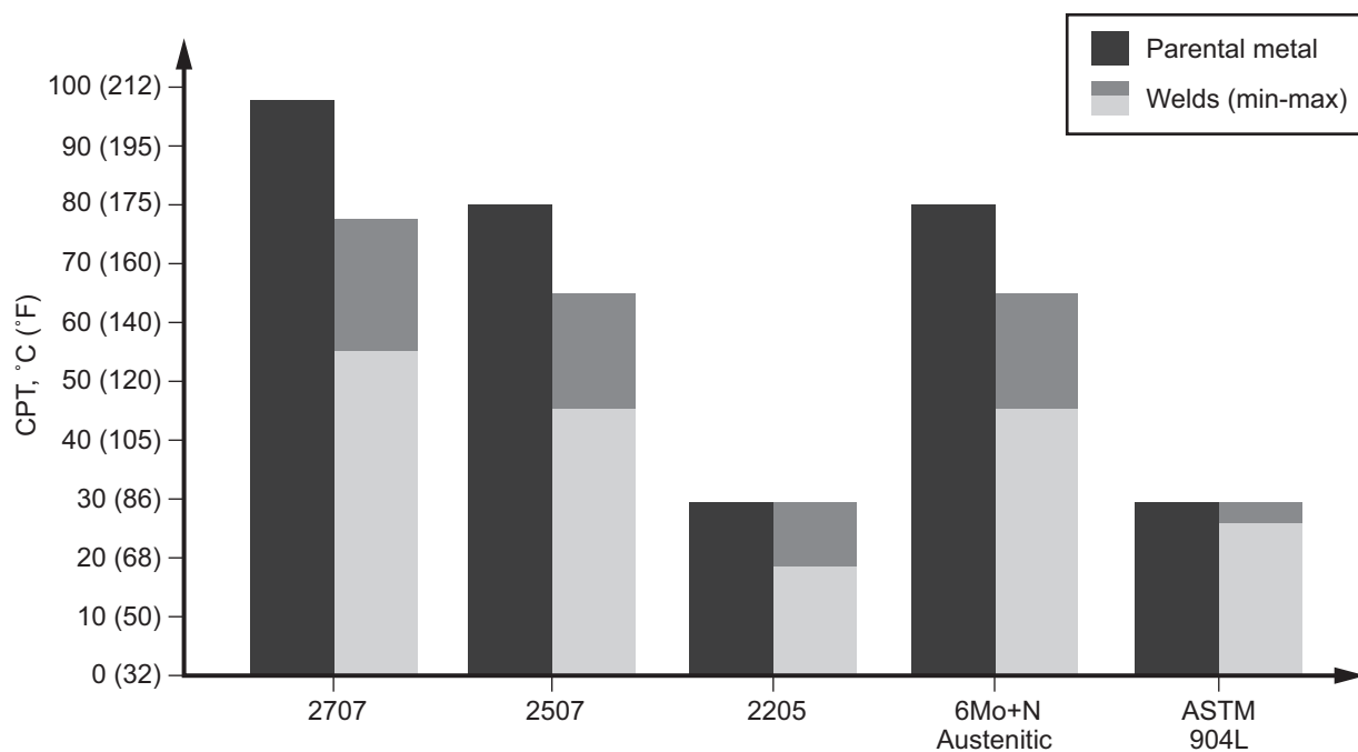
Figure 5—CPT for 22 % Cr, Super and Hyper DSSs Alloys Compared to Austenitic SS Alloys in 6 % FeCl 3 , ASTM G48 Test Method A [8]
