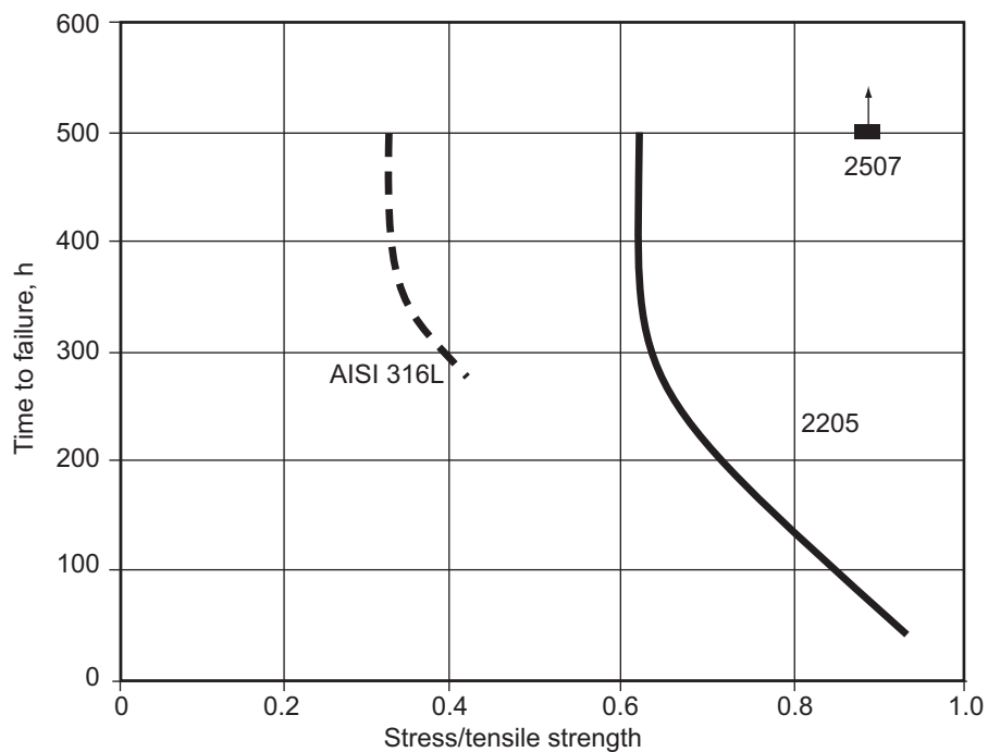
Figure 9—Results of SCC Tests of 22 % Cr and 25 % Cr DSSs Alloys Compared to Austenitic SS Alloys in Constant Load Tests in 40 % CaCl 2 , 1.5 pH at 100 °C with Aerated Test Solution [8]
