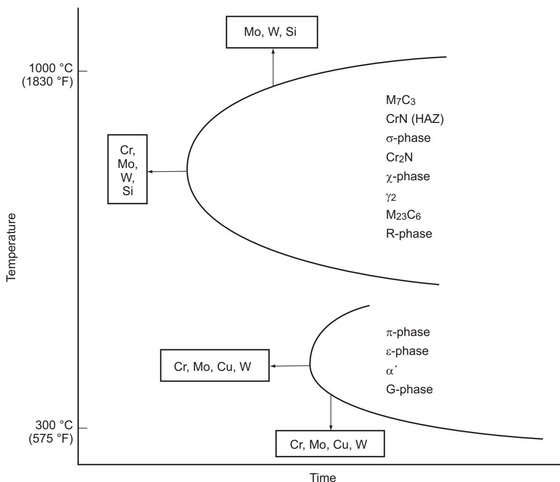
Figure 2—Possible Precipitations in DSSs [2]
