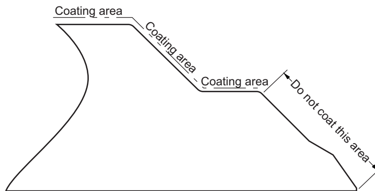
Figure L.3—Weld End
