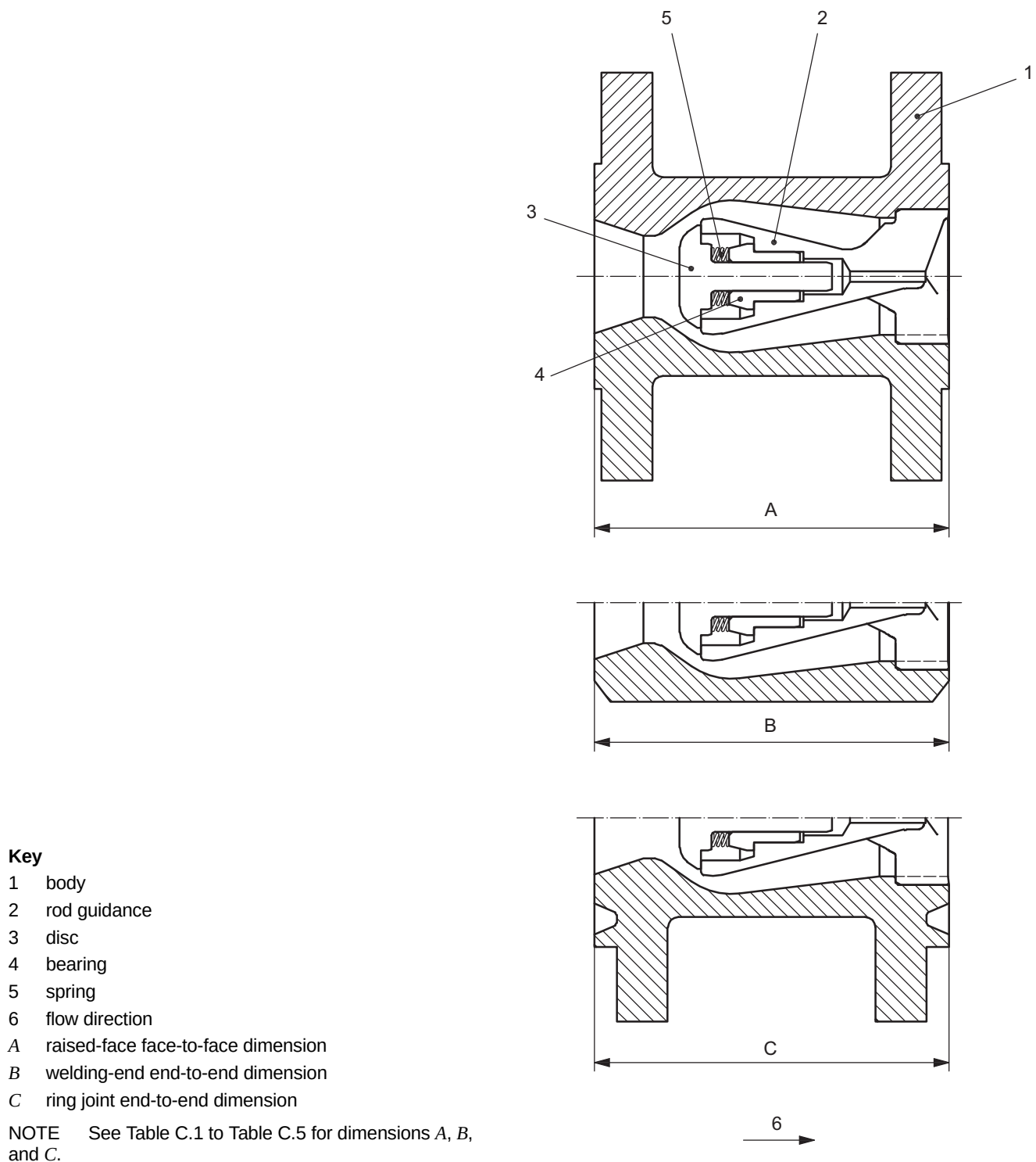
Figure B.12—Axial Flow Check Valve
