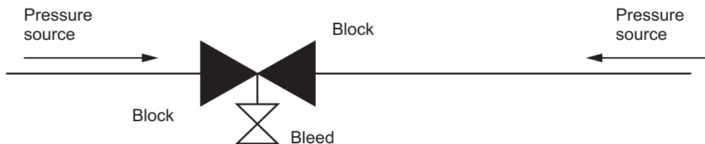
Figure K.4—Double Block and Bleed—Type B
