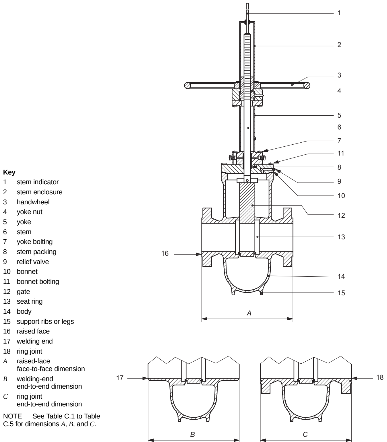
Figure B.2—Slab-gate/Through-conduit Rising-stem Gate Valve
