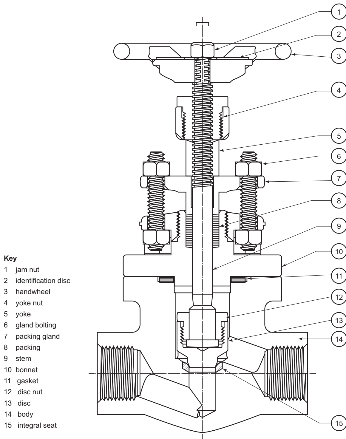
Figure E.5—Outside Screw and Yoke Globe Valve
