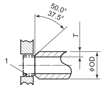
c) Beveled End for Welding
