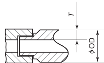
b) Socket-welded End
