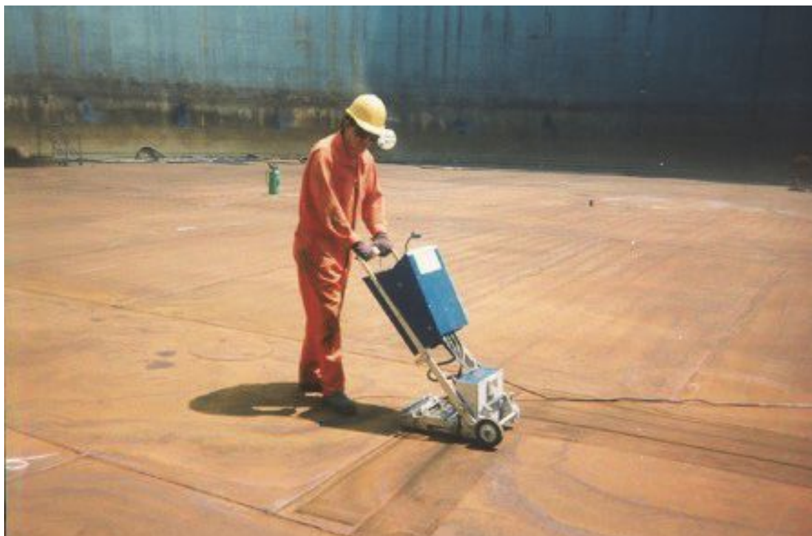
Figure A.2—MFL Scanner
