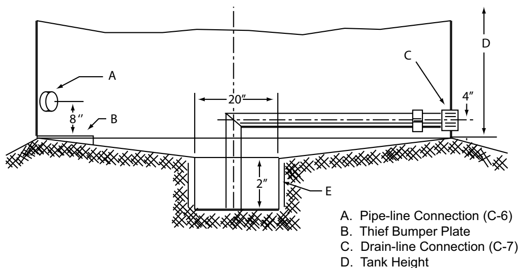
Figure 2—Type A (Unskirted) Cone Bottom
