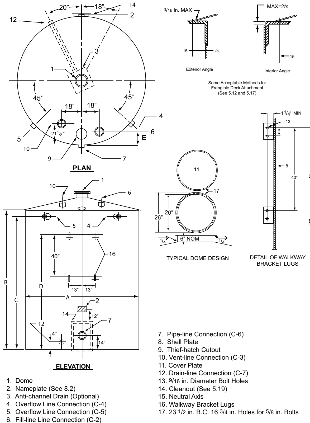
Figure 1—Tank Dimensions
