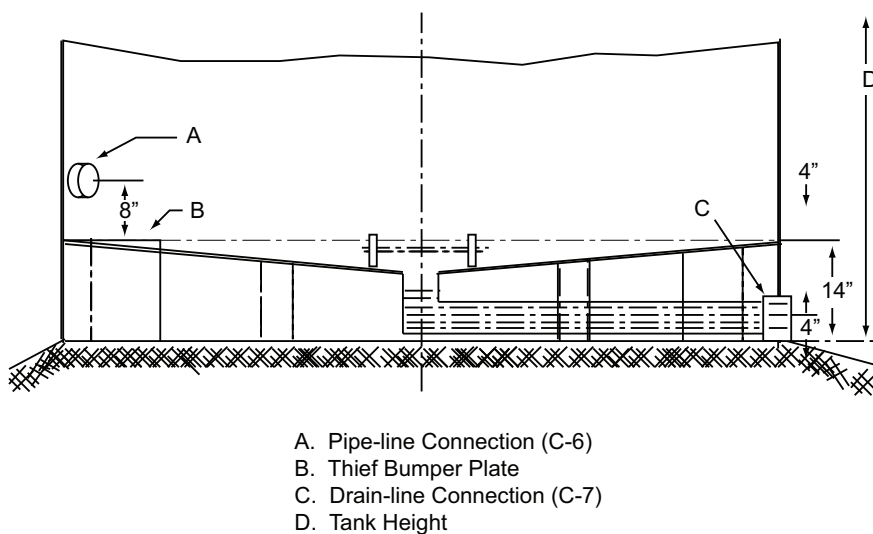
Figure 3—Type B (Skirted) Cone Bottom
