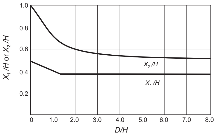
Figure EC.9—Center of Action for Effective Forces
