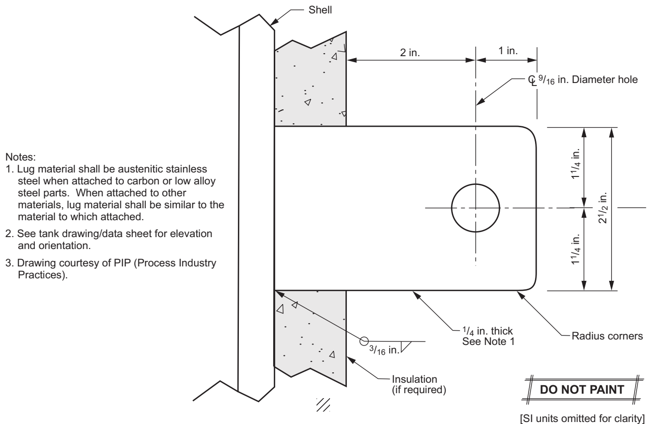
Figure 5.23—Grounding Lug
