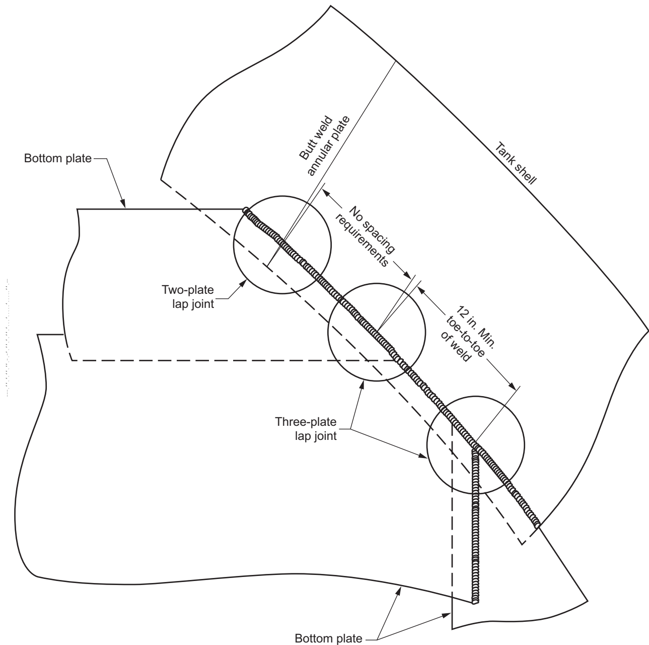
Figure 5.3d—Spacing of Three-Plate Welds at Annular Plates
