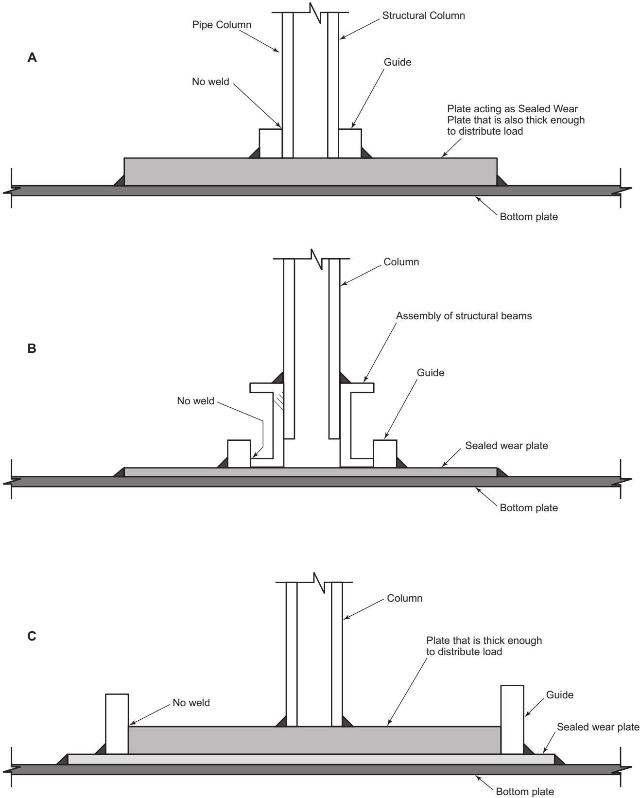
Figure 5.26—Some Acceptable Column Base Details
