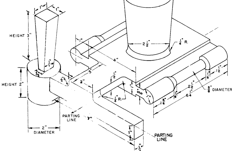
FIG. 2a Double Horizontal Full-Web Type Test Bars
