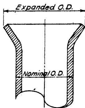
FIG. 2 Single Flare
