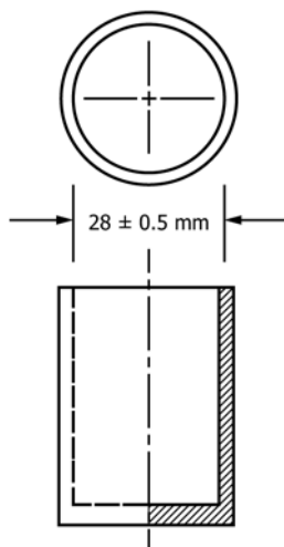
FIG. 2 Density Cup (25 \pm 0.03 cm 3 )
