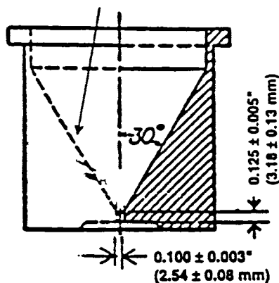
FIG. 1 Flowmeter Funnel
