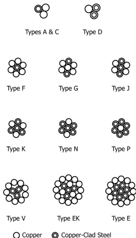
FIG. 1 Standard Types of Composite Conductors
