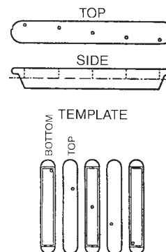
FIG. 1 Method of Sampling Lead by Sawing
