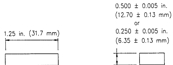
FIG. 4 Transverse Rupture Test Specimen
