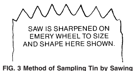
FIG. 3 Method of Sampling Tin by Sawing
