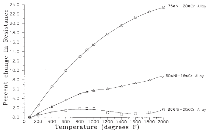
FIG. X1.1 Nominal Percent Change in Resistance with Temperature
