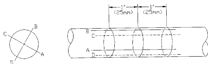
FIG. A4.1 Circumferential and Axial Scribe Lines for the Determination of Contractile Strain Ratio
