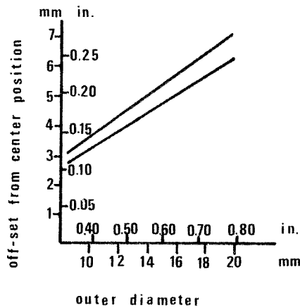
FIG. X2.2 Lamb-Wave Longitudinal Flaw Testing. Transducer Off-set Positioning as Function of Tube Outer Diameter
