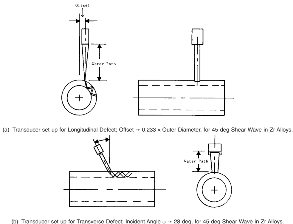
FIG. A3.1 Shear Wave Test for Longitudinal and Transverse Defects
