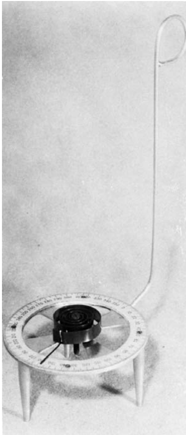
FIG. 1 Spiral Coil
