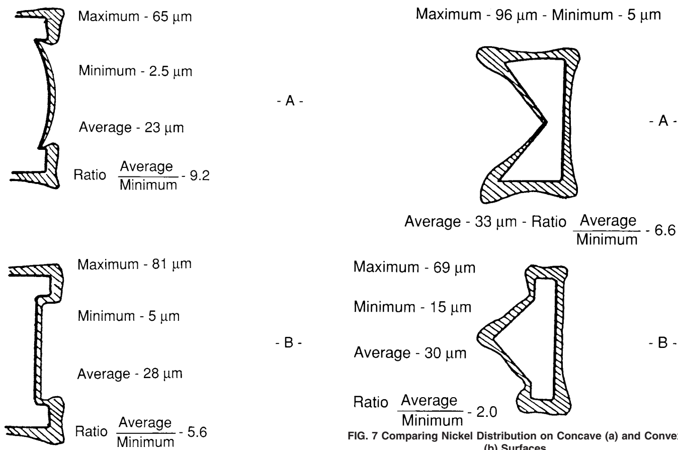
FIG. 6 Improving Nickel Thickness Distribution (Average/Minimum Thickness Ratio) by Rounding Corners
