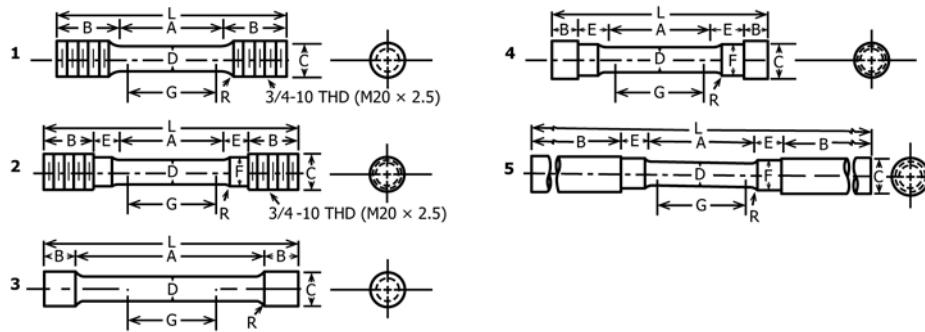
Dimensions, in.
