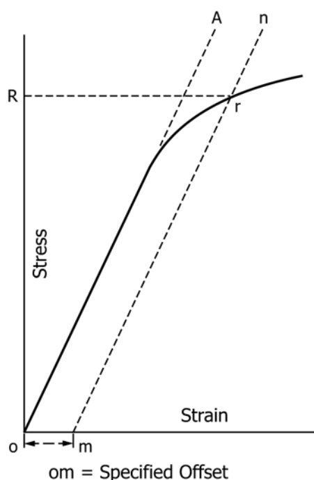
FIG. 16 Stress-Strain Diagram for Determination of Yield Strength by the Offset Method
