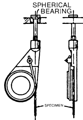
FIG. 5 Snubbing Device for Testing Wire
